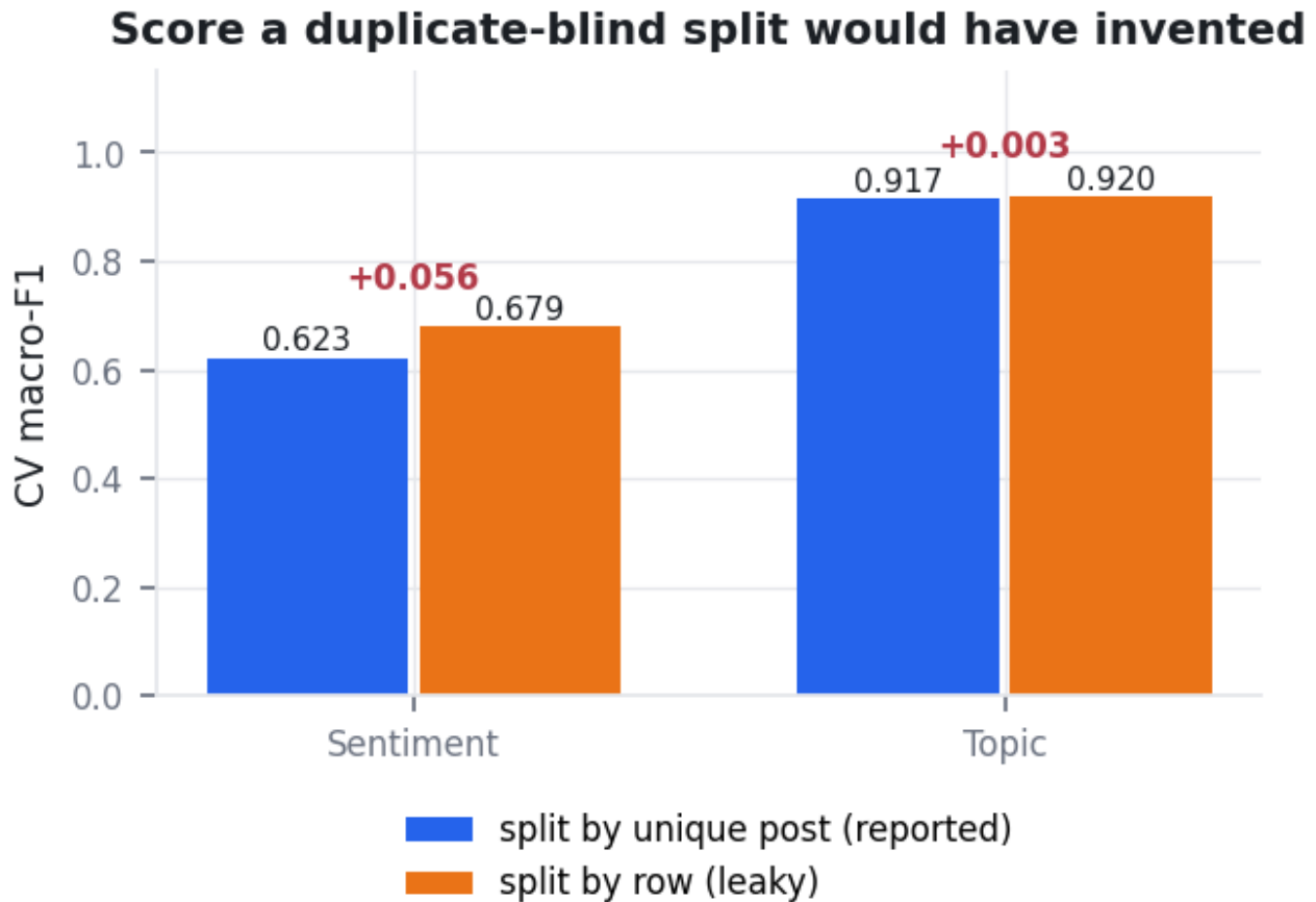
Figure 2. The same pipeline scored two ways. The orange bars are what a duplicate-blind evaluation would have reported.
