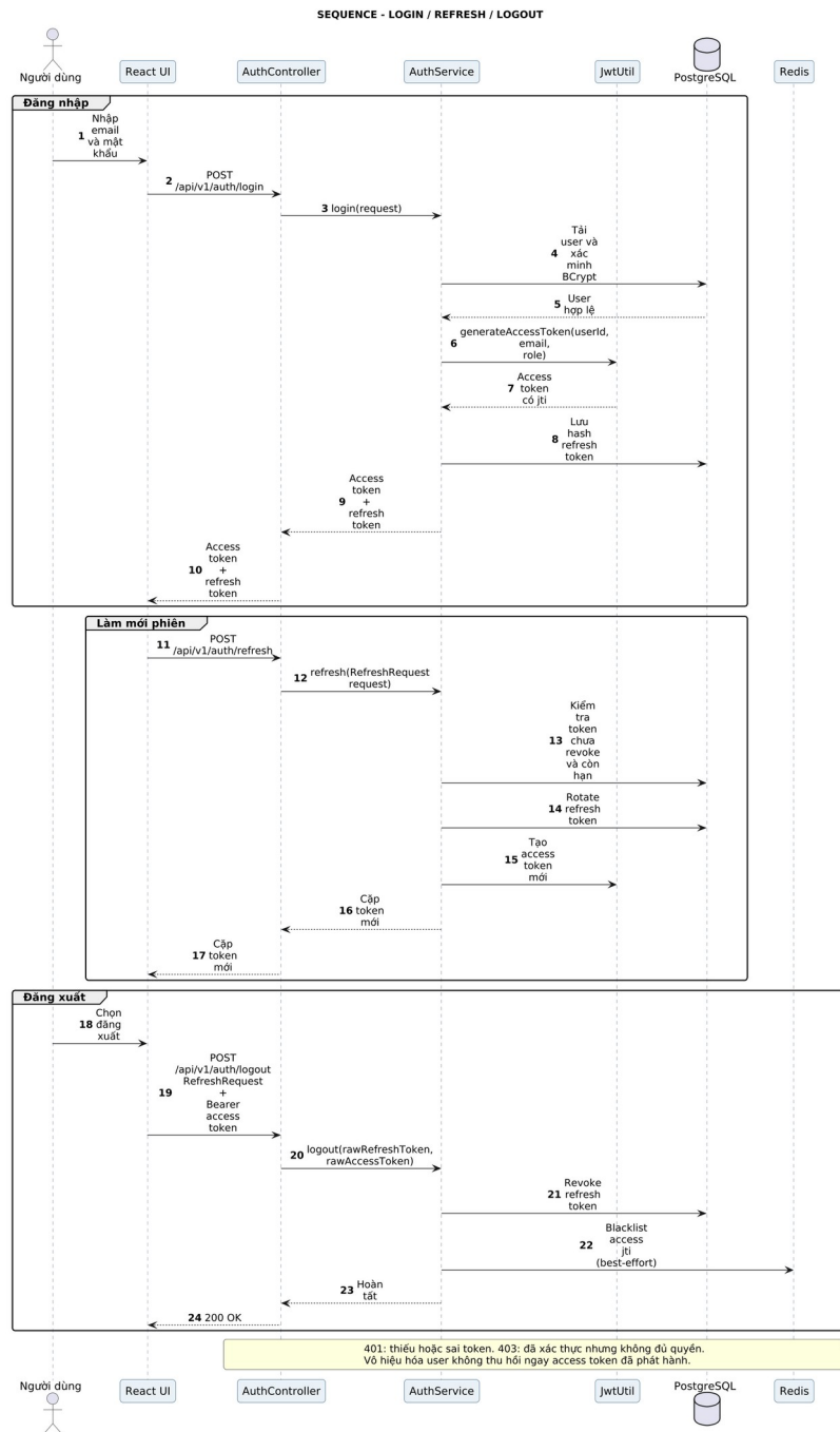
UML 4.1. Sequence Auth
