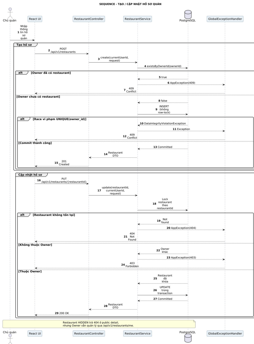
UML 4.2. Sequence Restaurant
