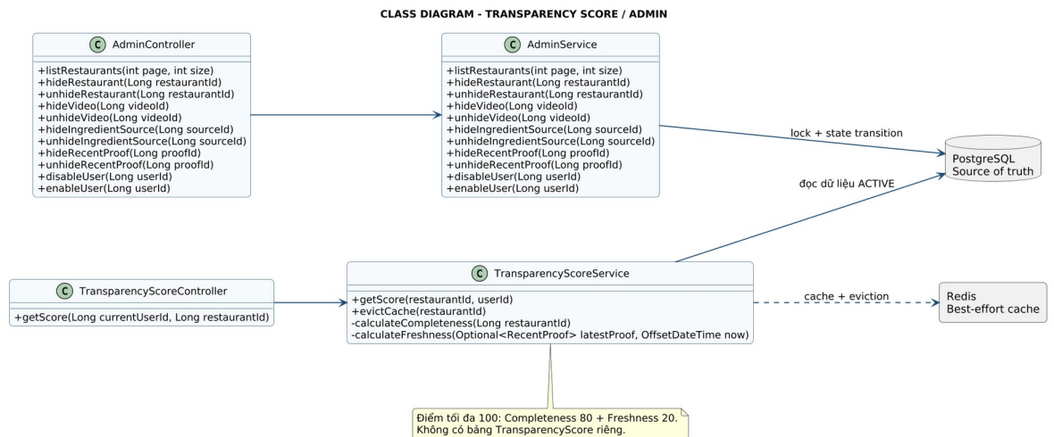
UML 3.7. Class diagram Score/Admin
