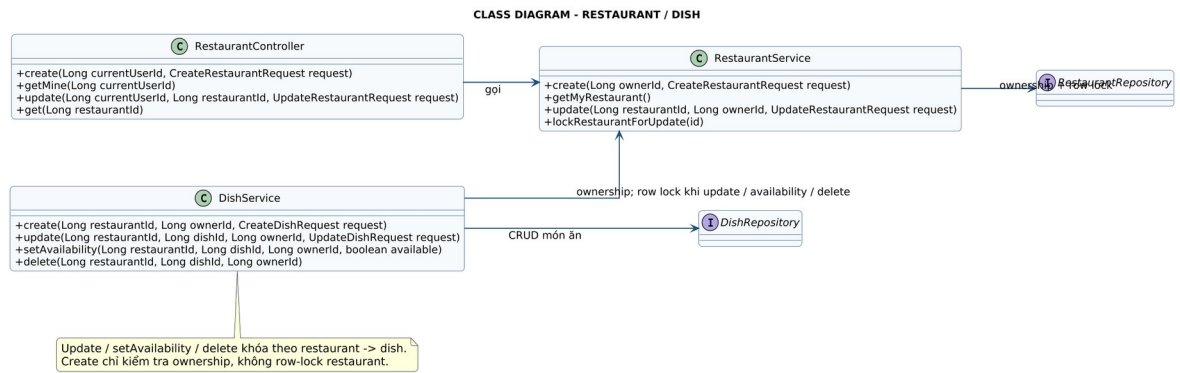
UML 3.5. Class diagram Restaurant/Dish
