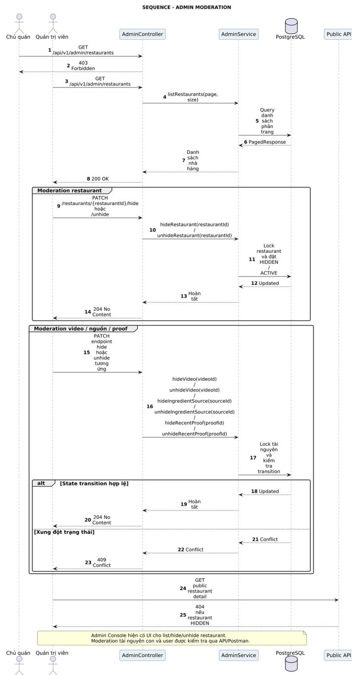
UML 4.5. Sequence Admin
