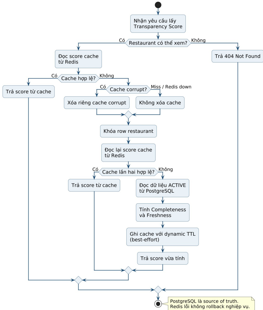
UML 4.4. Activity Transparency Score
