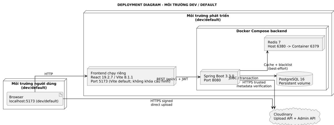
UML 5.1. Deployment diagram
