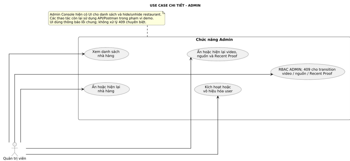
UML 2.3. Use case Admin
