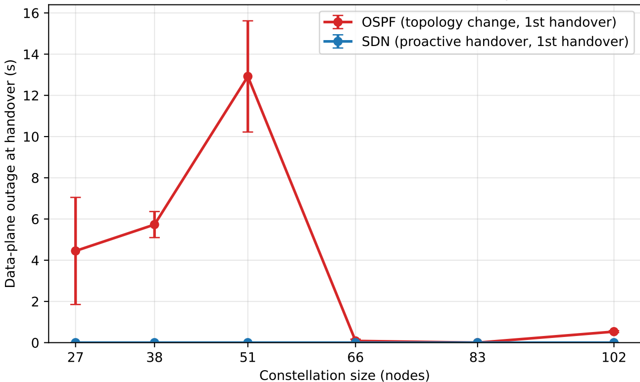
Handover black-hole duration — first handover per run
