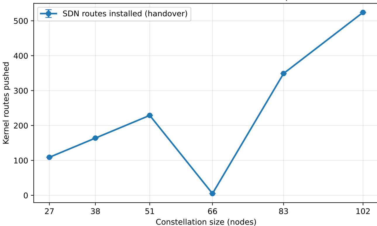
Incremental install size at first handover per run
