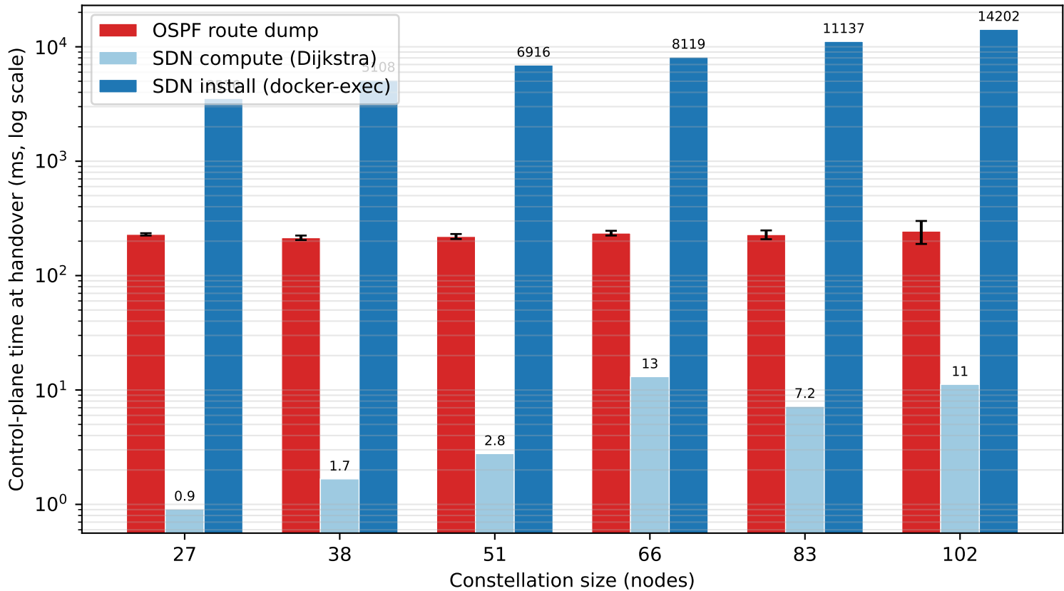
Handover control-plane cost (first handover per run)
