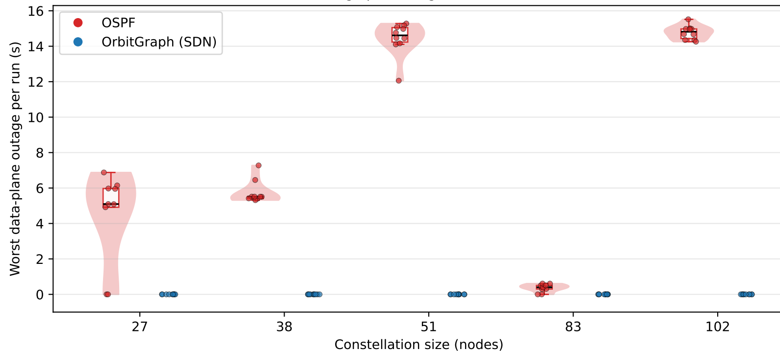
Coverage-preserving GSL handovers
