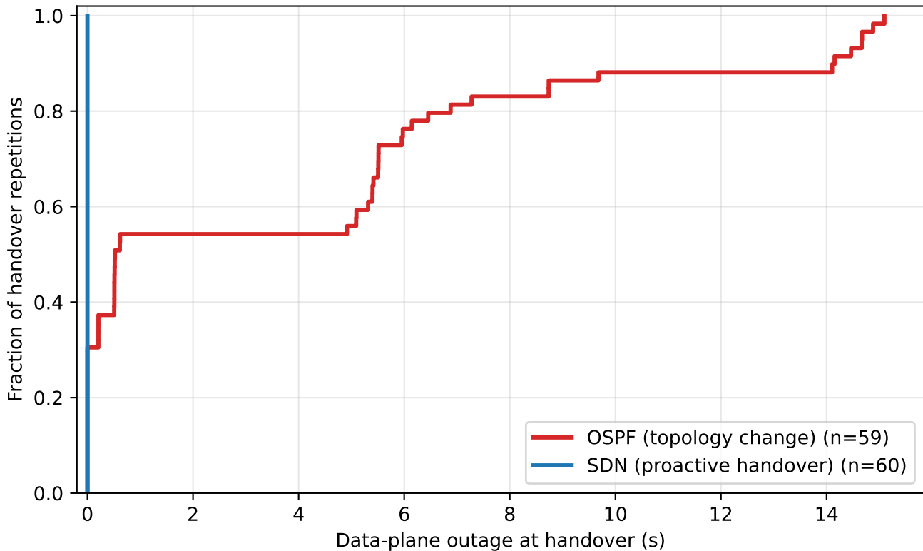
Handover outage ECDF (all constellation sizes pooled)
