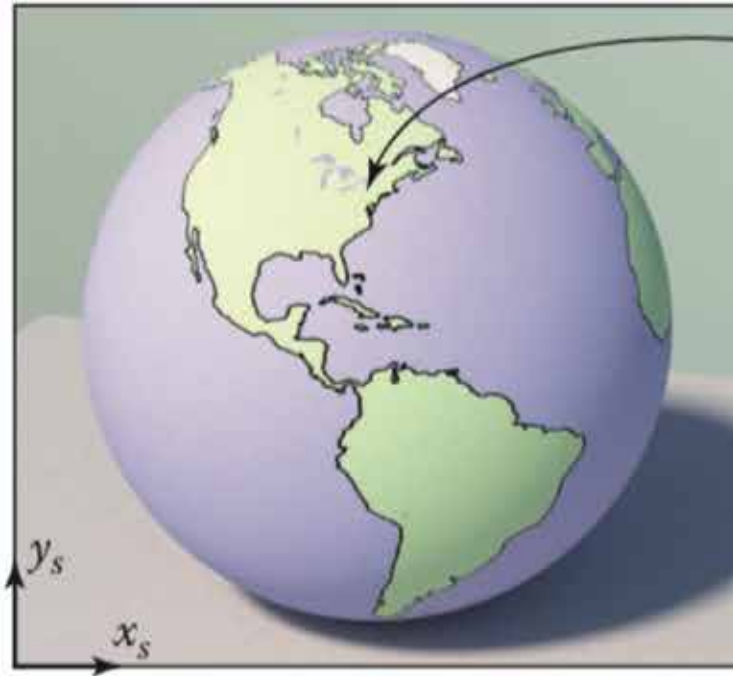
Image space
