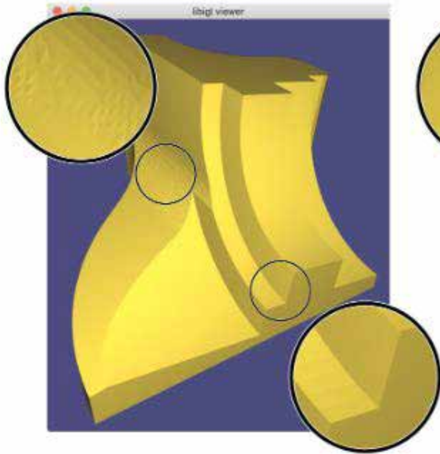
Per-Face Normals
