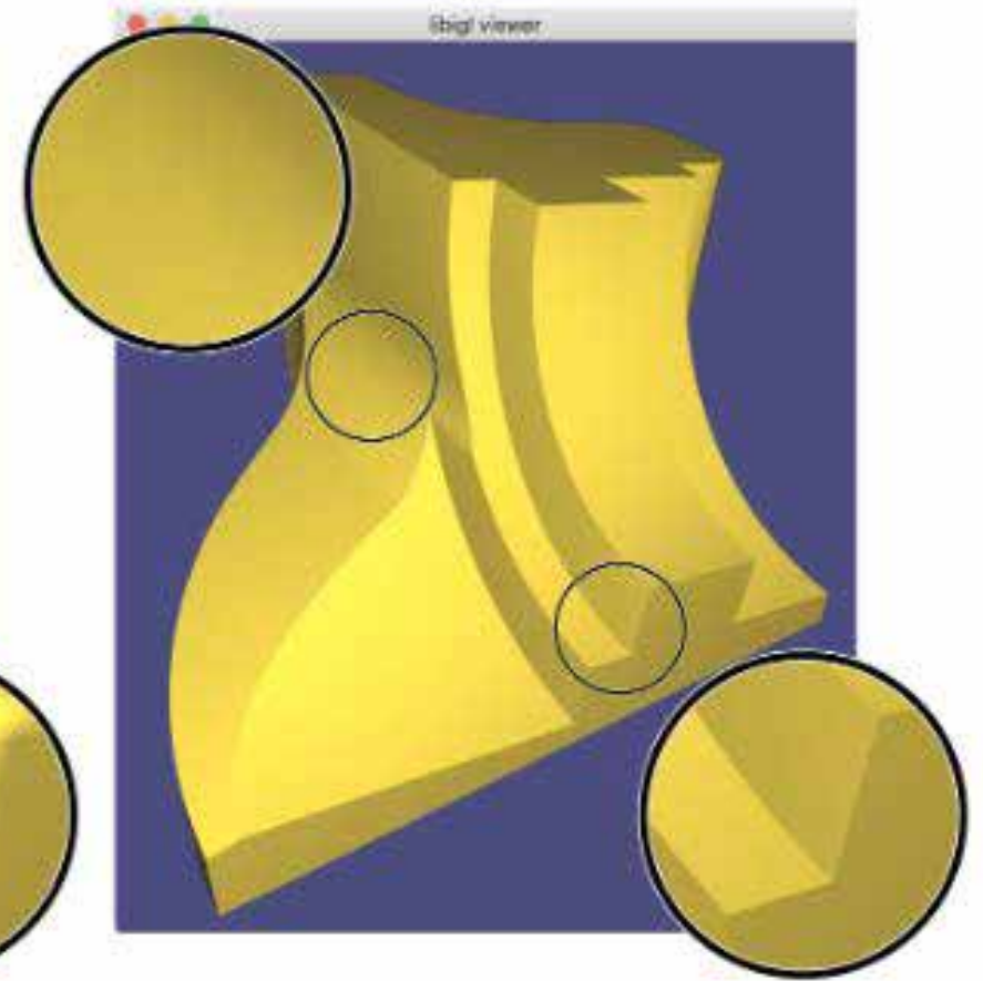
Per-Corner Normals
