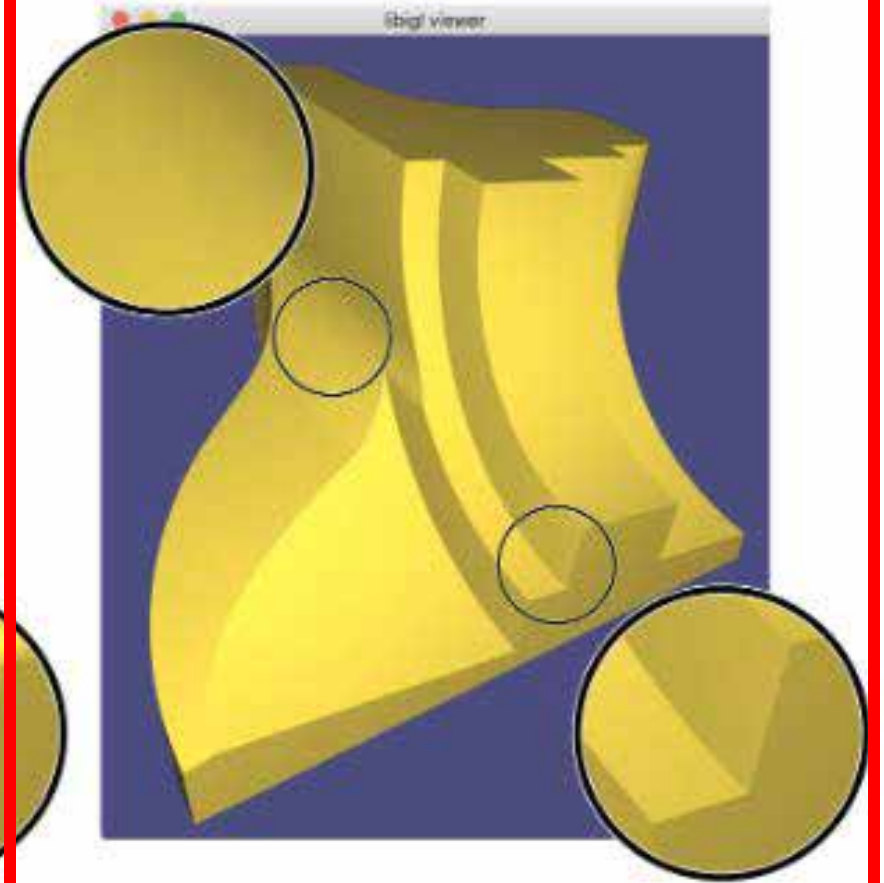
Per-Corner Normals
