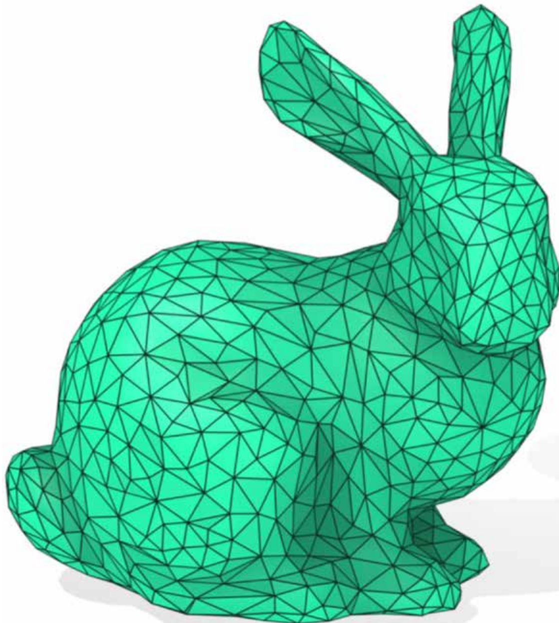
Mesh
