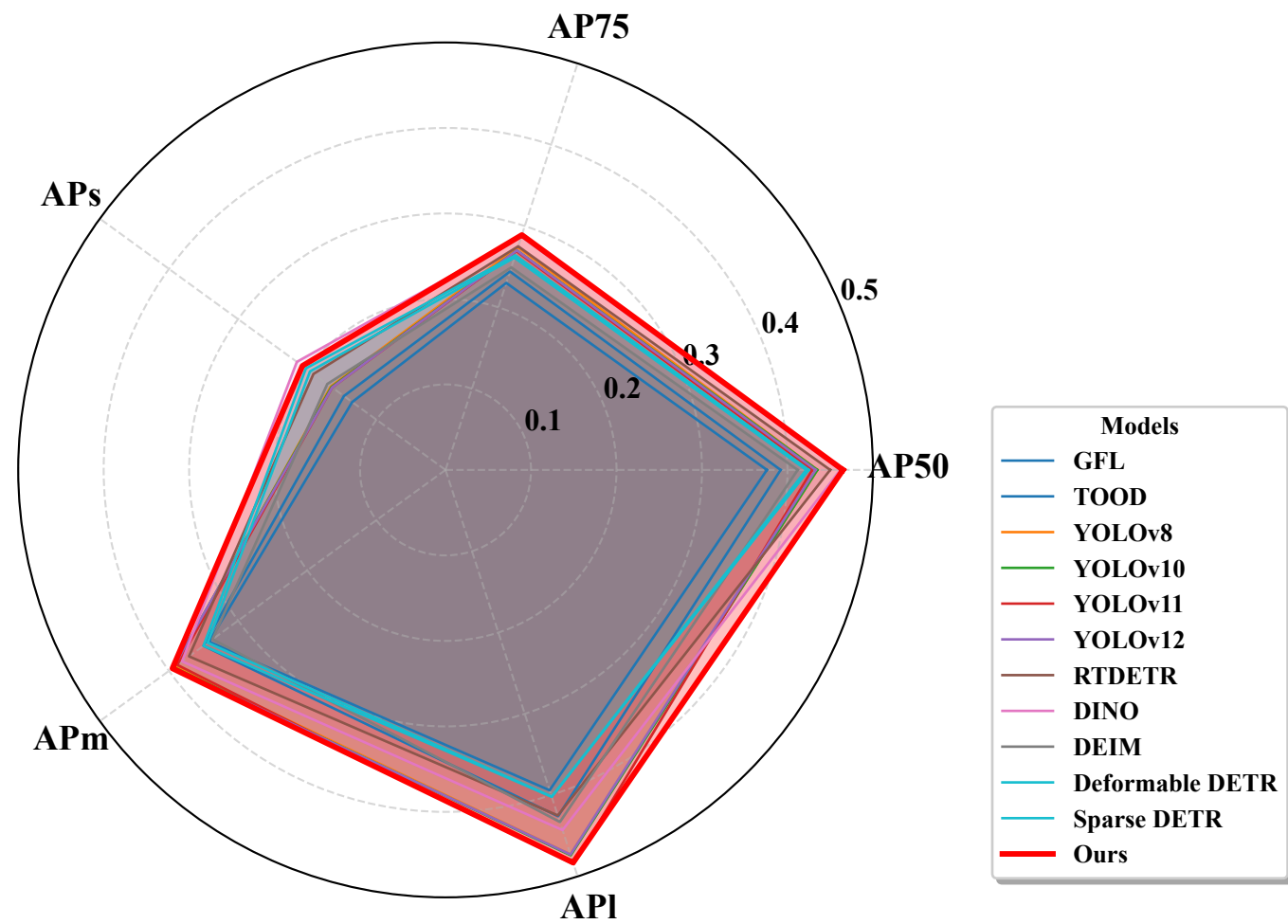
(a) Comprehensive AP Performance
