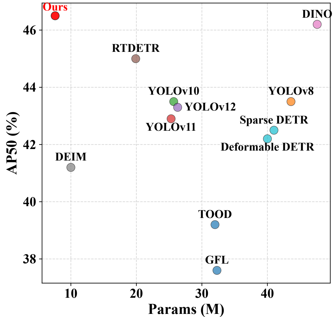
(b) Trade-off between AP50 and Params(M)
