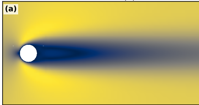
S-only — |\mathbf{u}|
