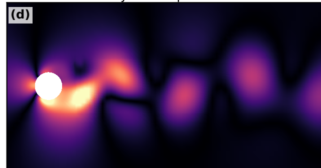
Proposed Specialist MoE — pressure error
