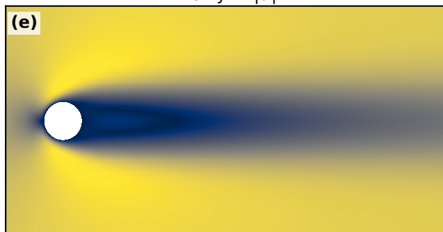
T2-C — |\mathbf{u}|
