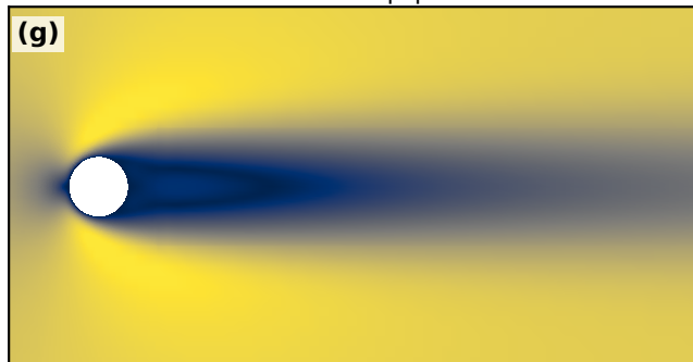
T2-C — |\mathbf{u}|
