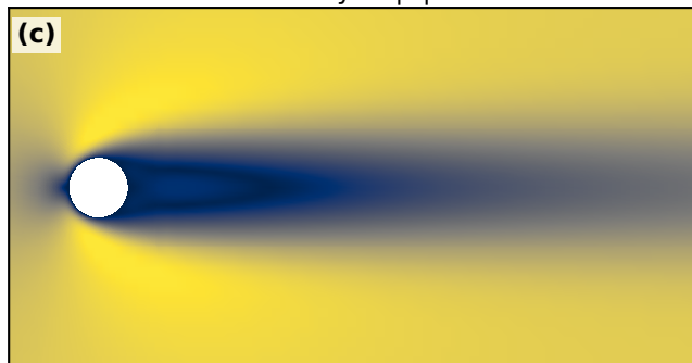
H-only — |\mathbf{u}|
