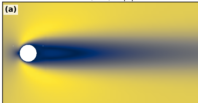
S-only — |\mathbf{u}|
