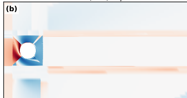
S-only — p
