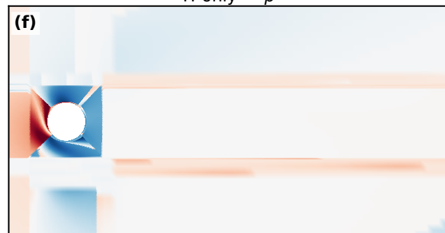
T2-C — p
