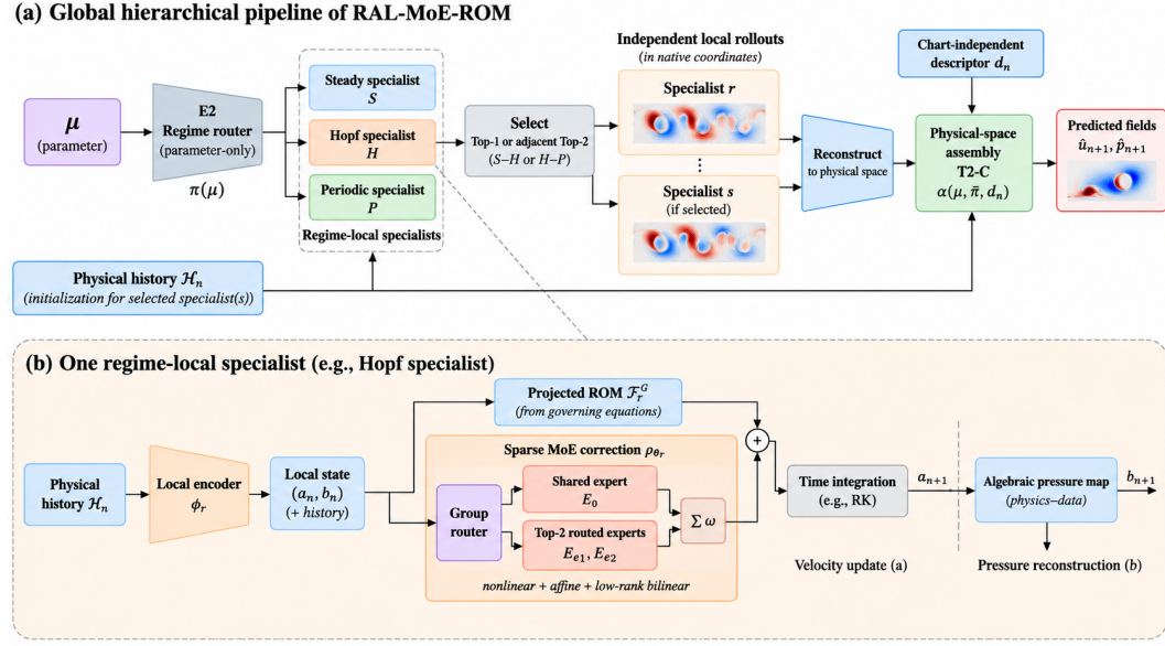
Figure 1: Hierarchical routing in RAL-MoE-ROM. (a) Parameter-only E2 selects one specialist or an admissible adjacent pair. Physical history initializes native charts and supplies T2-C’s descriptor d_n (history-to-assembly line), not E2. Independent rollouts are reconstructed before Top-1 identity output or Top-2 physical-space fusion, without fused-state feedback. (b) Within the selected group, shared and Top-2 experts contribute in parallel. Only velocity is integrated; pressure is reconstructed algebraically from updated velocity and local features (auxiliary connection omitted). Flow thumbnails are schematic, not experimental results.
