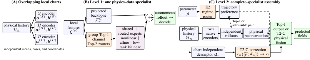
Figure 1: Overview of RAL-MoE-ROM. Sparse routing acts within each regime-local specialist, while parameter-only regime routing selects complete local models. Physical-history descriptors condition only T2-C, which combines independently evolved specialists after reconstruction in the common physical space.
