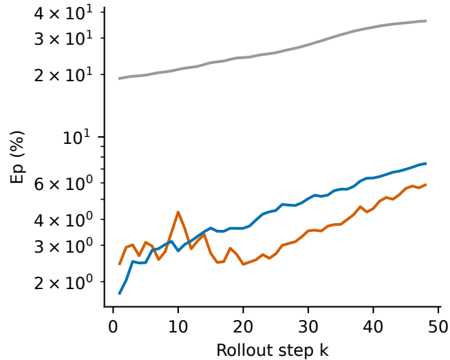
Circular Periodic · 12 aligned held-out windows · common POD-reconstructed truth
