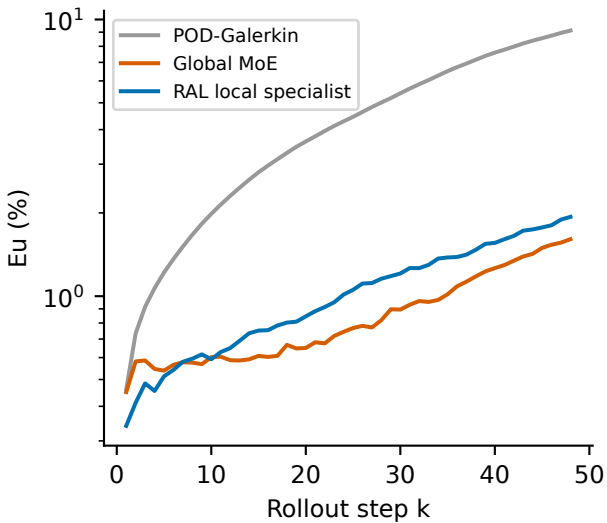
Circular Periodic · 12 aligned held-out windows · common POD-reconstructed truth
