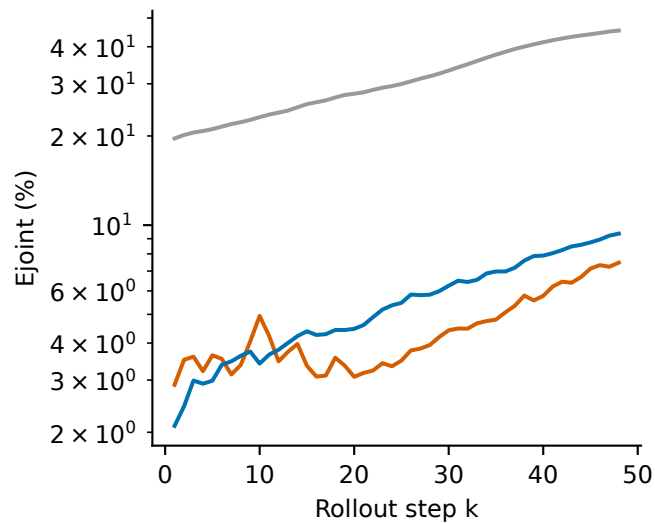
Circular Periodic · 12 aligned held-out windows · common POD-reconstructed truth
