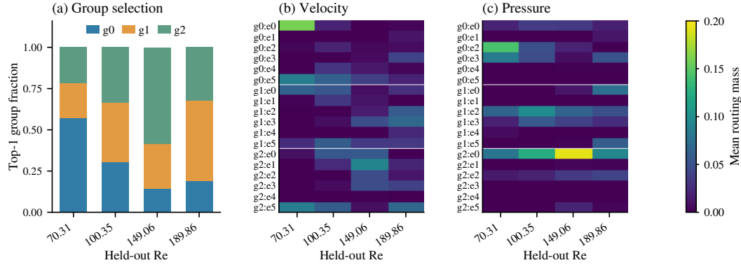
Figure 6: Parameter-dependent internal routing of the frozen Circular Periodic specialist. (a) Top-1 group-selection frequencies. (b,c) Mean routed-expert mass for velocity and pressure, respectively. Records are collected at the first integration stage of each output step over 13 windows per Reynolds number. Expert labels are local to each group and channel; the shared component is not shown.
