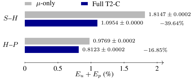
Figure 2: Full-window Square comparison over three paired gate seeds. All local candidates and E2 are fixed; bars show mean and sample standard deviation.
