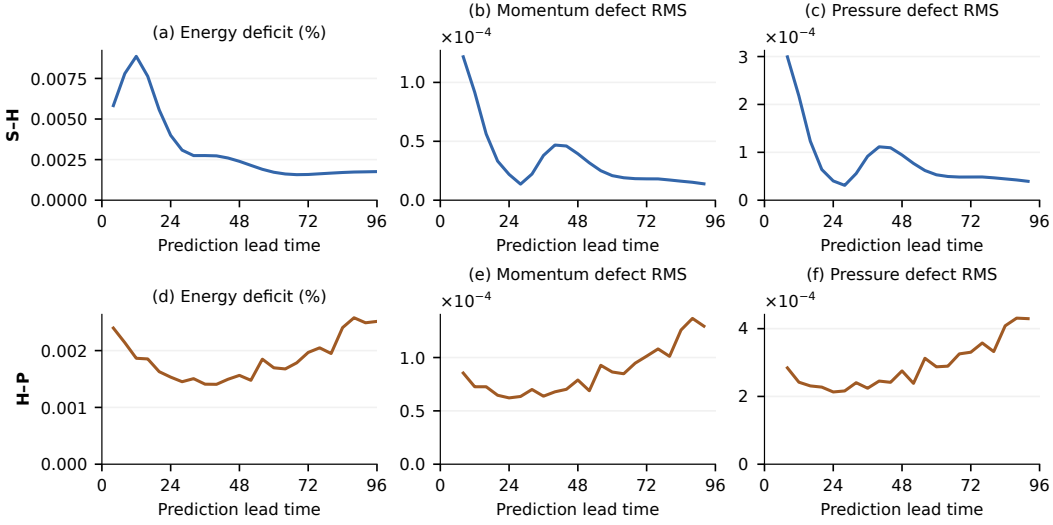
Figure 5: Additional effects of Square T2-C fusion with the 24-neighbor initial stencil. Rows correspond to S-H (top) and H-P (bottom); columns show normalized energy deficit d_E in percent, momentum-defect RMS, and pressure-defect RMS. Each curve averages all 16 windows at each prediction lead time. Energy uses steps 1–24; residuals use steps 2–23. Residual RMS is computed over the interior wake before window averaging. The energy deficit is relative to weighted candidate energies, not reference-energy error; residual defects are not total residuals. Axes use panel-specific scales.
