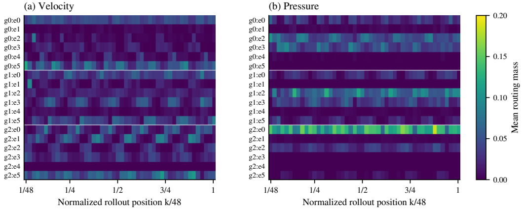
Figure 7: Periodic routed-expert mass along autonomous rollouts. Each column averages records at the same output step across 52 windows; all routed experts are retained. The horizontal coordinate k/48 denotes normalized prediction position, not physical oscillation phase. Masses include the routed-component scaling and exclude the shared expert.
