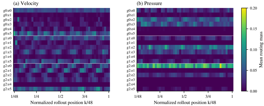
Figure 9: Routed-expert mass versus autonomous rollout position for the circular-cylinder Periodic specialist. Each column averages the routing decision at the corresponding reduced time step over the 52 fixed held-out windows, and all routed experts are retained. The horizontal coordinate is the normalized prediction position k/48 and is not interpreted as physical oscillation phase.
