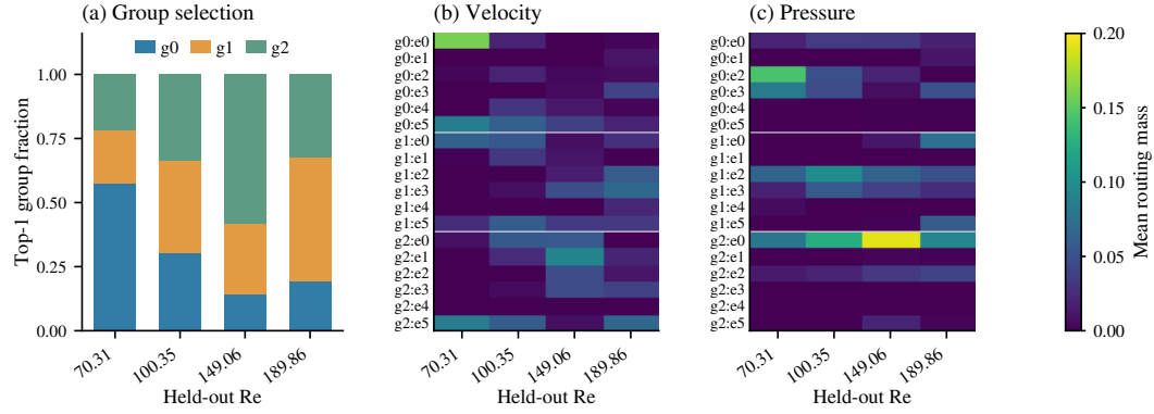
Figure 8: Internal routing of the circular-cylinder Periodic specialist on held-out autonomous roll-outs, recorded once per reduced time step at the first integration stage. (a) Top-1 group-selection frequencies. (b,c) Mean routed-expert mass for the velocity and pressure channels. Expert identifiers are local to the corresponding specialist, group, and channel and are not assigned physical labels.
