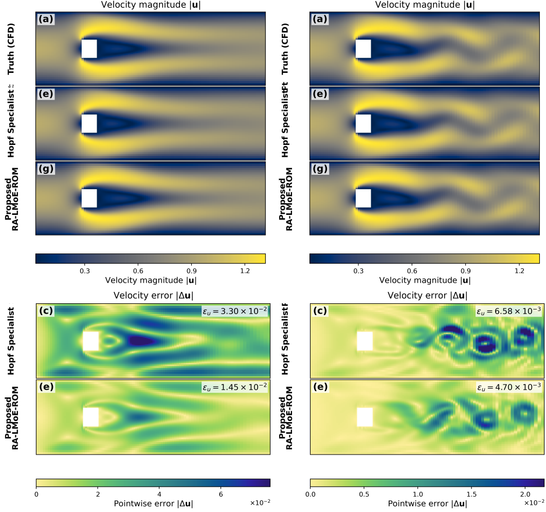
Figure 3: Representative centered-square overlap predictions for S-H (left) and H-P (right). T2-C combines independently evolved local predictions only after reconstruction in physical space. The displayed examples illustrate the corresponding reduction in velocity-field error; complete velocity and pressure comparisons are reported in Appendix G.
