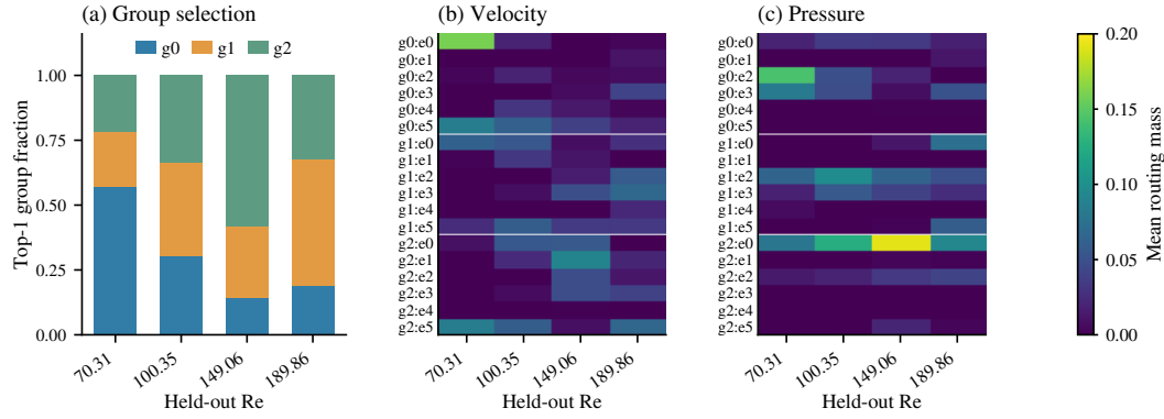
Figure 5: Internal routing of the circular-cylinder Periodic specialist on held-out autonomous rollouts, recorded once per reduced time step at the first integration stage. (a) Top-1 group-selection frequencies. (b,c) Mean routed-expert mass for the velocity and pressure channels. Expert identifiers are local to the corresponding specialist, group, and channel and are not assigned physical labels.
