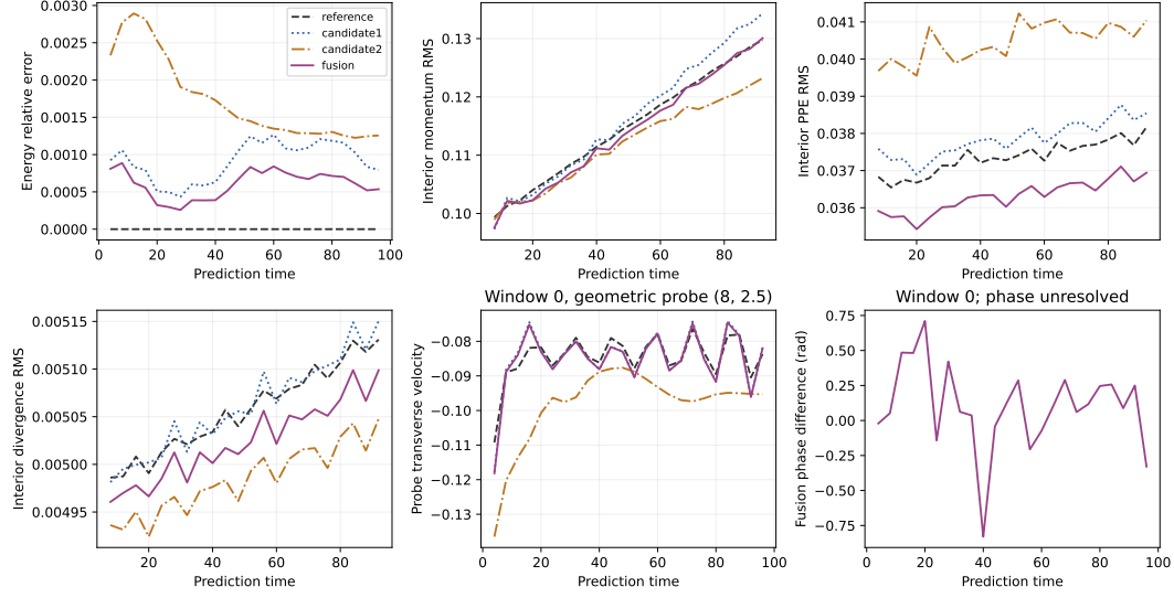
Figure 11: H-P diagnostics under the same protocol. Candidate 1 is Periodic and candidate 2 is Hopf. The first four panels average all 16 windows; the probe and phase panels show the first frozen window, which is unresolved by the stated phase screen.
