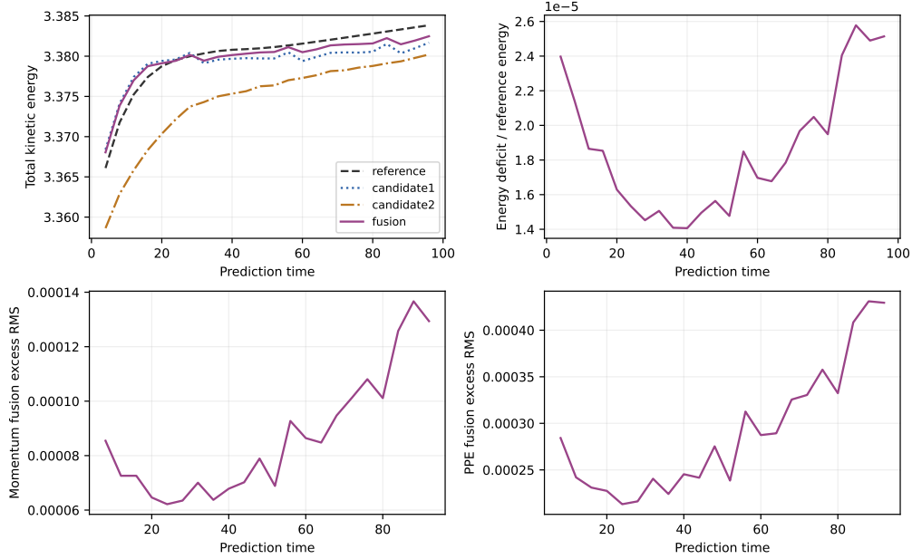
Figure 12: Actual kinetic energy and additional fusion defects averaged over all windows. The energy deficit is measured relative to the weighted candidate energies, normalized by reference energy; it is not the energy error. Momentum and pressure excesses are differences from the weighted candidate residuals, not the total fused residuals.
