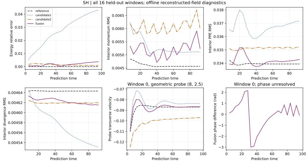
Figure 10: S-H diagnostics: the first four panels average all 16 windows; the last two show the first frozen window, not a best-case selection. Candidate 1 is Steady and candidate 2 is Hopf. Reference is POD-reconstructed CFD. The unresolved phase trace is descriptive only.
