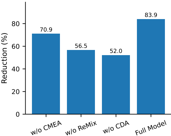
FADE
