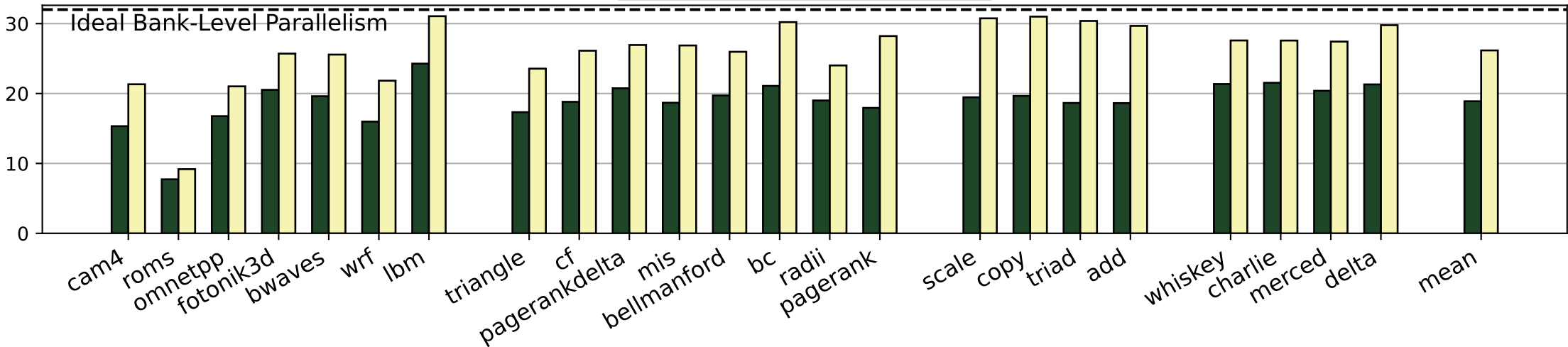
Bank Level Parallelism
