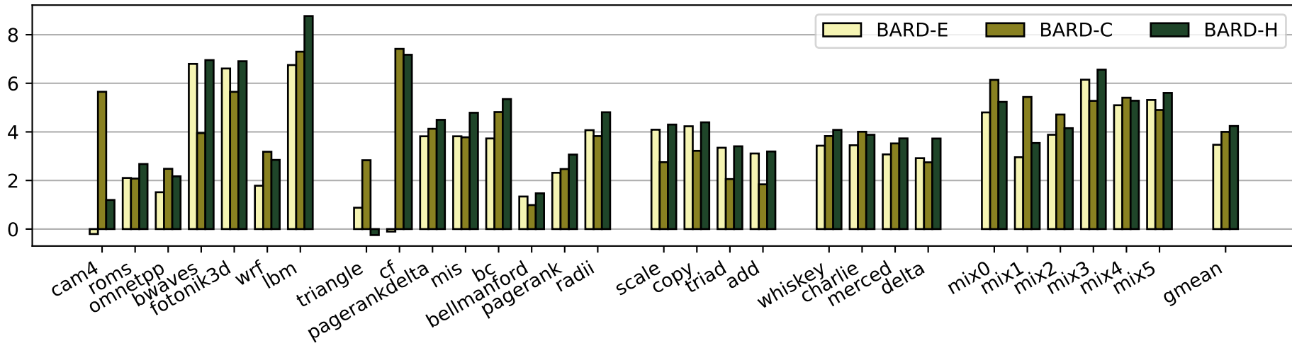
Speedup (%)
