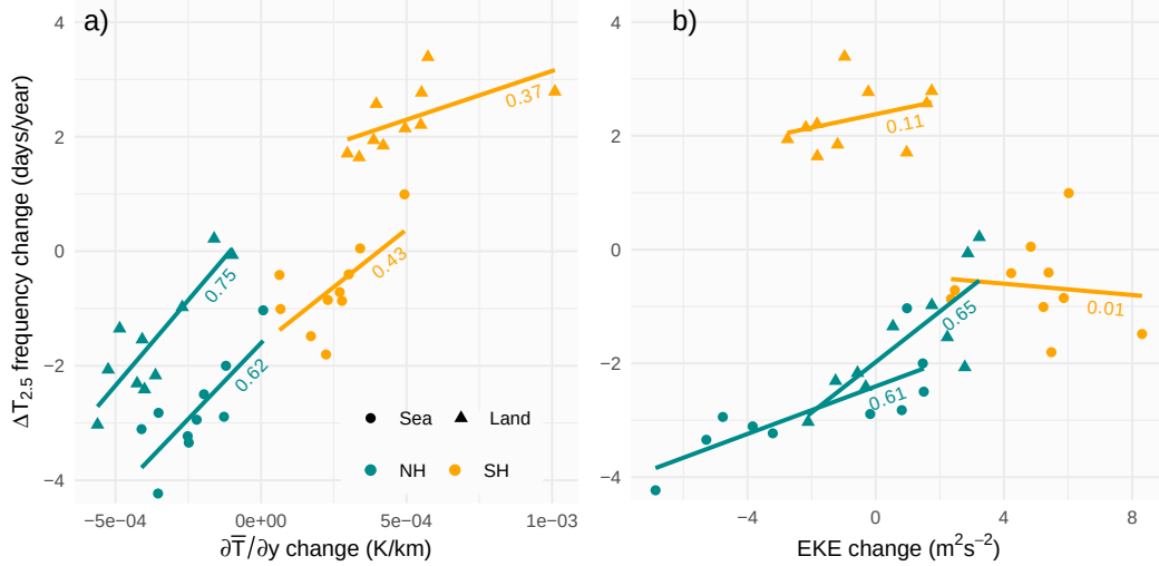
Figure 4: Mean change in the mean \Delta T_{2.5} frequency and a) mean meridional temperature gradient \partial \bar{T} / \partial y and b) the EKE of the storm track for SSP5-8.5 (2080-2100) compared with the historical period (1980-2000) for each model. Values are calculated for the Northern ( 25^\circ to 65^\circ ) and Southern ( -25^\circ to -65^\circ ) Hemispheres and over sea (circles) and land (triangles). Each solid line corresponds to a linear regression for each hemisphere.
