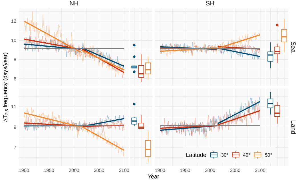
Figure 2: Multimodel yearly mean frequency of \Delta T_{2.5} for the historical period (1900-2014) and SSP5-8.5 (2015-2100) over land and sea for different 2° wide latitude bands centered at 30, 40 and 50°. The grey line represents the climatological frequency for 1979-2014, equal to 9.125 \Delta T_{2.5} /year. On the right of each panel box plots of the intermodel distribution is shown for the period 2080-2100. In the boxplots the lower and upper hinges correspond to the first and third quartiles and the upper (lower) whisker extends to the largest (smallest) value no further than 1.5 * inter-quartile range. Outside the whiskers dots represents outliers.
