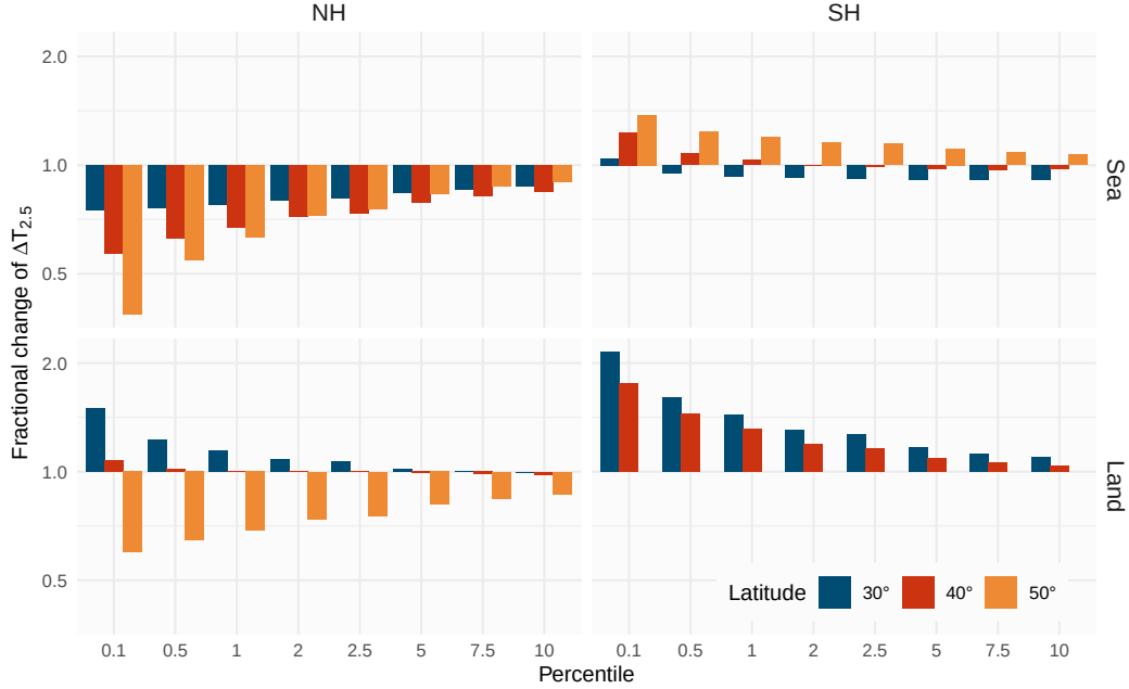
Figure 3: Fractional change in the frequency of strong \Delta T averaged between the years 2080-2100 under the SSP5-8.5 scenario compared to that averaged between 1980-2000 in the historical scenario, for different thresholds defined by their percentile value for each grid point and model calculated over the historical period (1979-2014).
