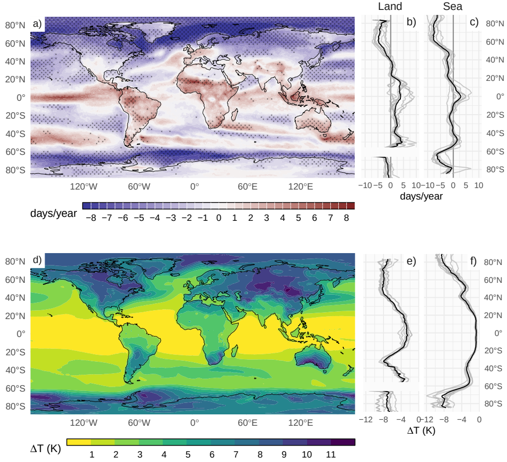
Figure 1: a) Multimodel mean change in the frequency of \Delta T_{2.5} (days/year, SSP5-8.5 2080-2100 minus Historical 1980-2000) and zonal mean change over b) land and c) sea, each grey line represents a model listed in Table 1 and a black line represents the multimodel mean. In a) dotted areas show where at least 90% of the models agree in the sign of change. d) \Delta T values associated with the 2.5 th percentile and zonal mean over e) land and f) sea.
