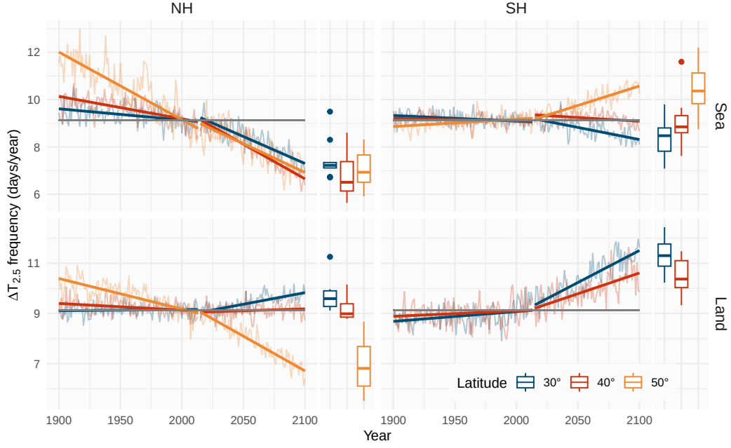
Figure 2: Multimodel yearly mean frequency of \Delta T_{2.5} for the historical period (1900-2014) and SSP5-8.5 (2015-2100) over land and sea for different 2^\circ wide latitude bands centered at 30^\circ , 40^\circ and 50^\circ . The grey line represents the climatological frequency for 1979-2014, equal to 9.125 \Delta T_{2.5}/\text{year} . On the right of each panel box plots of the intermodel distribution is shown for the period 2080-2100. In the boxplots the lower and upper hinges correspond to the first and third quartiles and the upper (lower) whisker extends to the largest (smallest) value no further than 1.5 * \text{inter-quartile range} . Outside the whiskers dots represents outliers.
