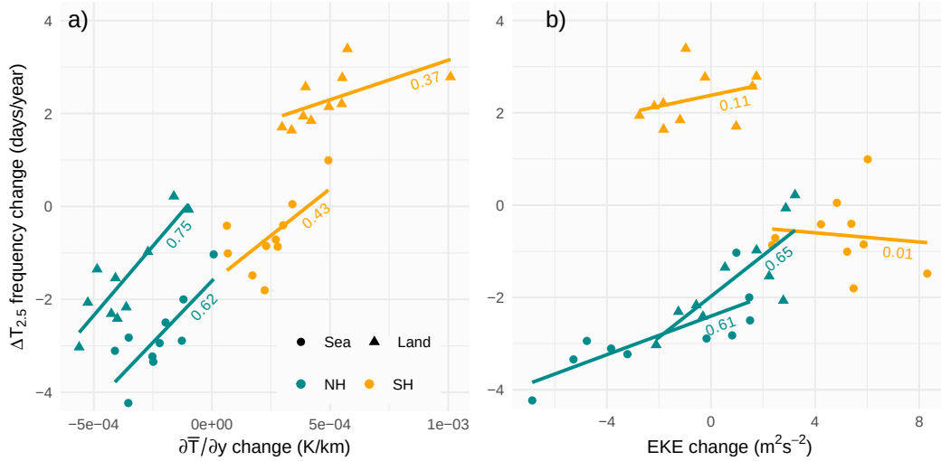
Figure 4: Mean change in the mean \Delta T_{2.5} frequency and a) mean meridional temperature gradient \partial \bar{T} / \partial y and b) the eddy kinetic energy of the storm track EKE for SSP5-8.5 (2080-2100) compared with the historical period (1980-2000) for each model. Values are calculated for the Northern ( 25^\circ to 65^\circ ) and Southern ( -25^\circ to -65^\circ ) Hemispheres and over sea (circles) and land (triangles). Each solid line corresponds to a linear regression for each hemisphere.
