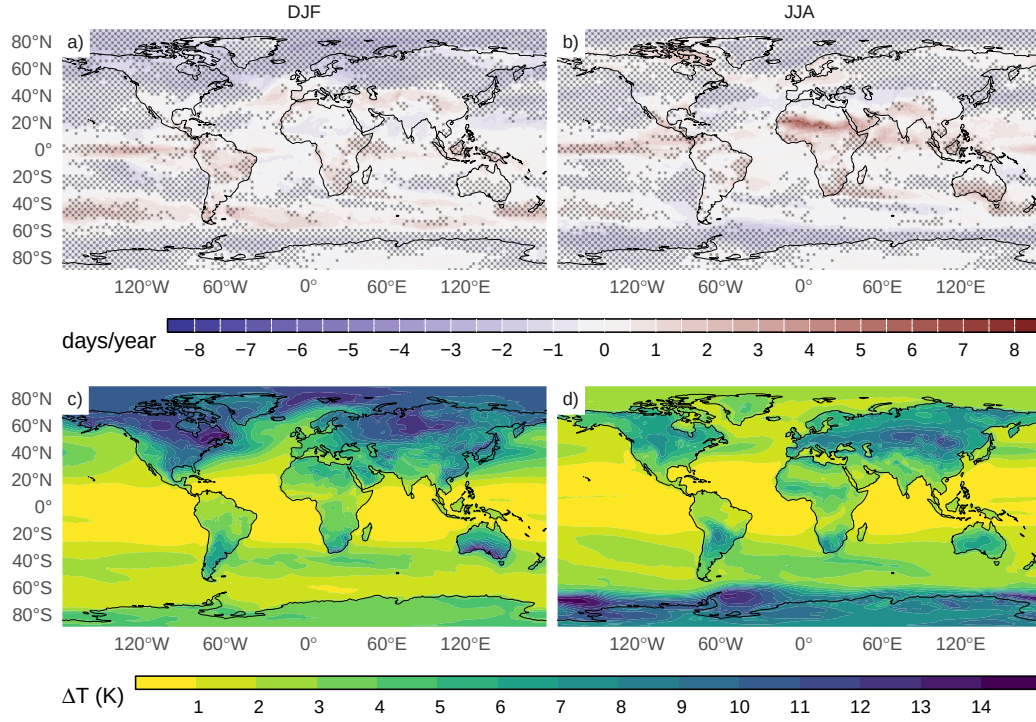
Figure S1: Multimodel mean change in the frequency of \Delta T_{2.5} (days/year, SSP5-8.5 2018-2100 minus Historical 1980-2000) for a) DJF and b) JJA and \Delta T values associated to the 2.5 percentile calculated for c) DJF and d) JJA. In a-b) dotted areas show where at least 90% of the models agree in the sign of change.
