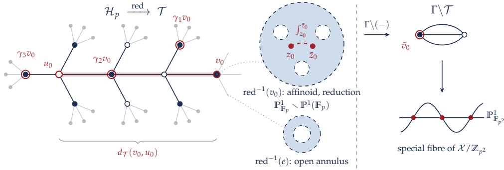
Figure 2: The Čerednik–Drinfeld uniformisation at a prime p . Left. Drinfeld’s upper half plane \mathcal{H}_p = \mathbb{P}_{\mathbb{C}_p}^1 \setminus \mathbb{P}^1(\mathbb{Q}_p) retracts onto the (p + 1) -regular Bruhat–Tits tree \mathcal{T} of \mathrm{PGL}_2(\mathbb{Q}_p) . The fibre of \mathrm{red} over a vertex is an affinoid with canonical reduction \mathbb{P}_{\mathbb{F}_p}^1 \setminus \mathbb{P}^1(\mathbb{F}_p) while over an open edge is an open annulus. Right. X_{\mathbb{Q}_{p^2}} \cong \Gamma \backslash \mathcal{H}_p . The finite graph \Gamma \backslash \mathcal{T} is the dual graph of the special fibre, whose components are \mathbb{P}_{\mathbb{F}_{p^2}}^1 meeting at ordinary double points.
