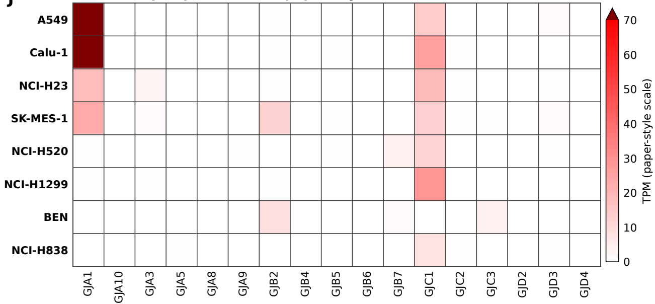
DepMap 24Q4 TPM (paper-style 0-70 scale; saturated)
