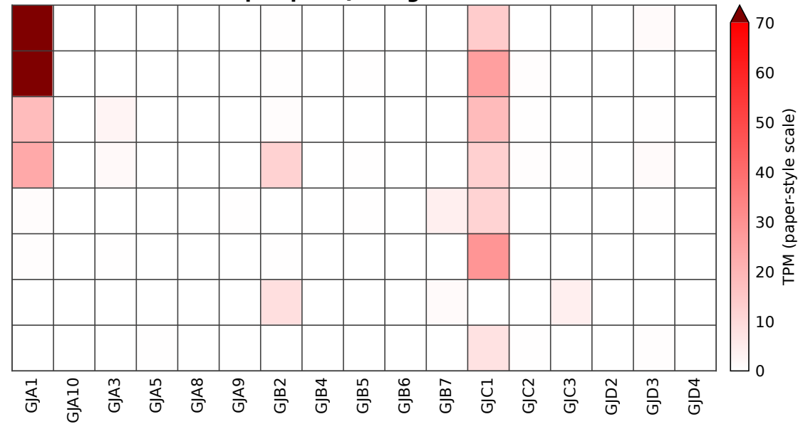
DepMap 24Q4 all-gene TPM
