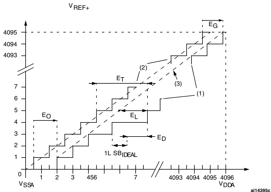
Figure 40. ADC accuracy characteristics
