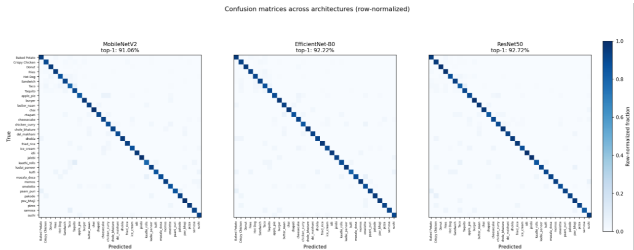
Figure 9. Row-normalized confusion matrices for all three architectures on the test set. All three show the same off-diagonal pattern.
