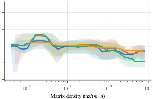
Row reordering
