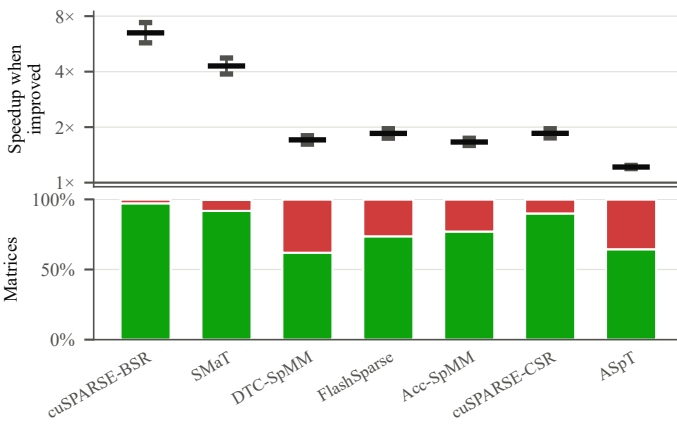
Scrambled matrices, symmetric reordering
