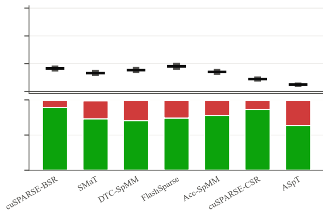
Scrambled matrices, row reordering
