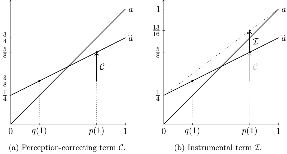
Figure 1: Decomposition in Example 1 with under-perception.
