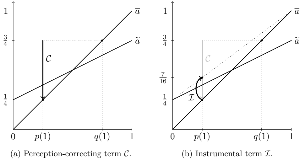
Figure 2: Decomposition in Example 1 with over-perception.
