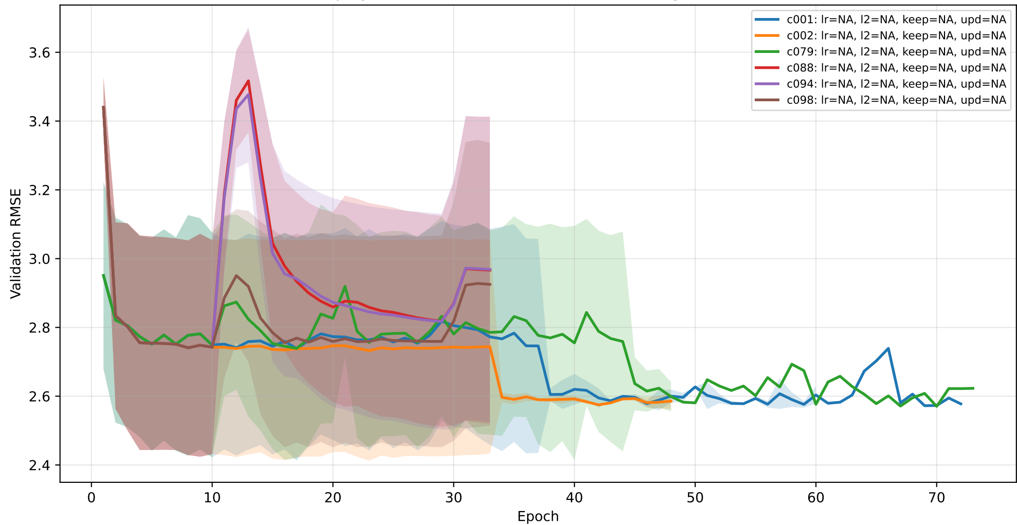
polynomial: ALE-Fréchet ablation learning curves
