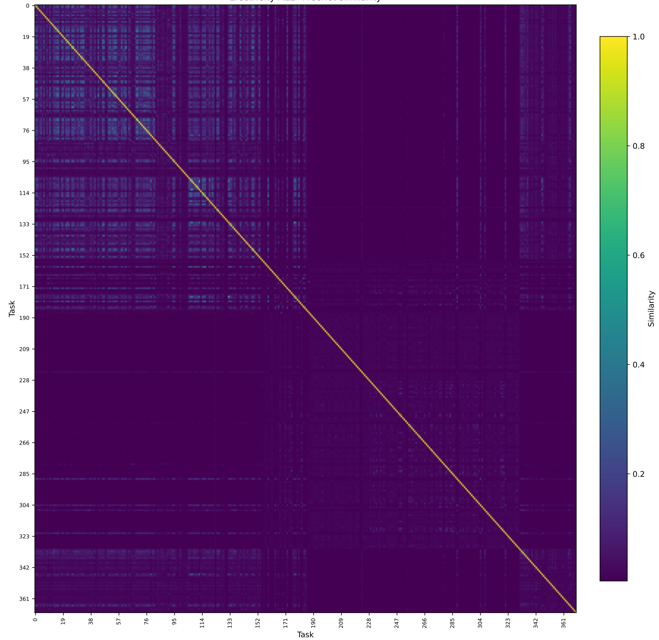
Electricity ALE--Frechet similarity
