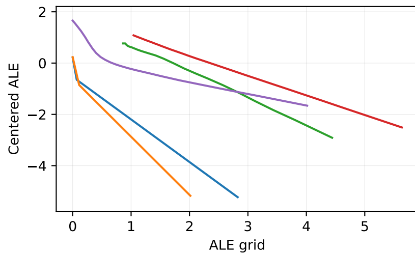
Latent feature 125
