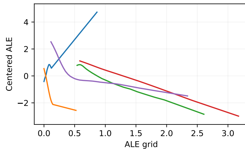
Latent feature 115
