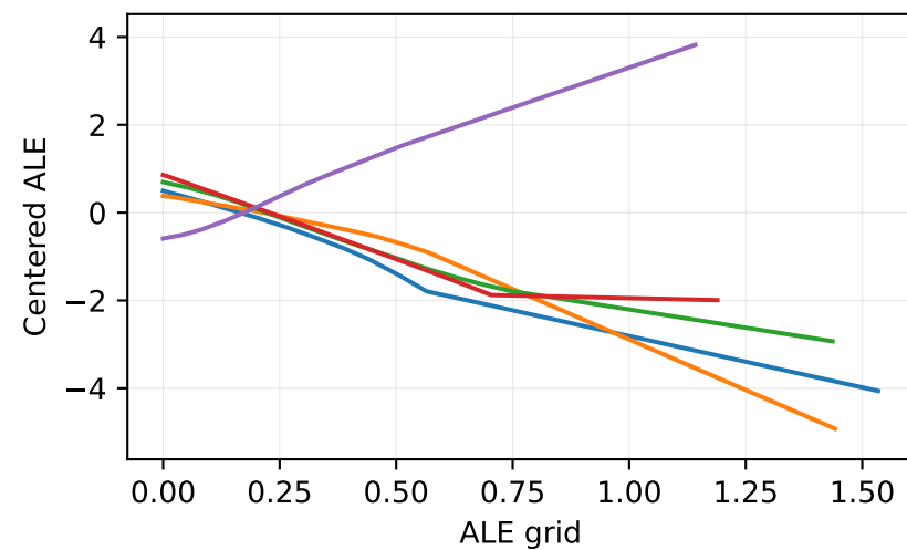
Latent feature 104
