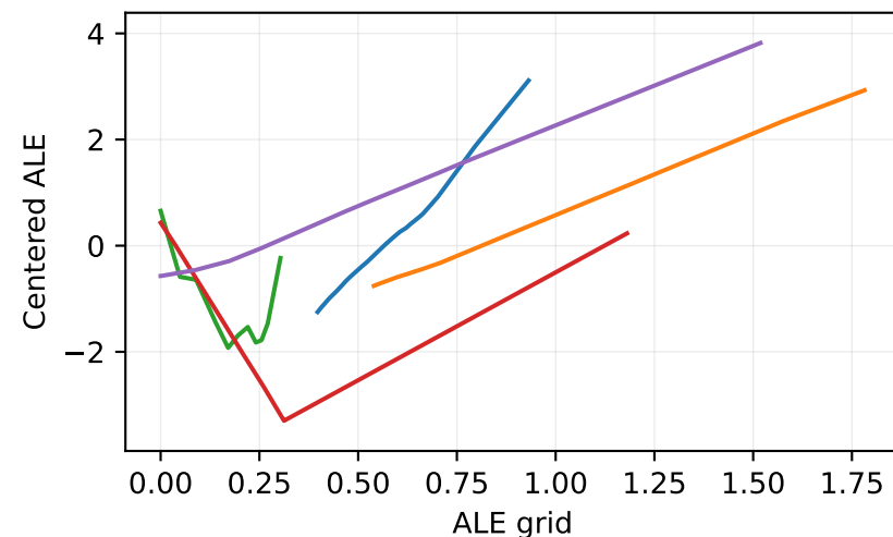
Latent feature 104
