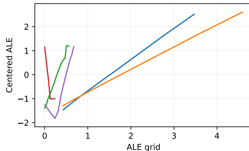
Latent feature 115
