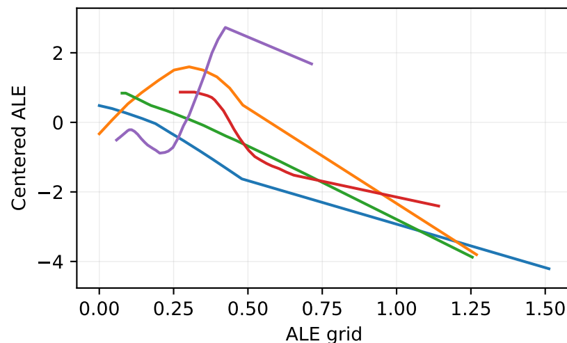
Latent feature 125
