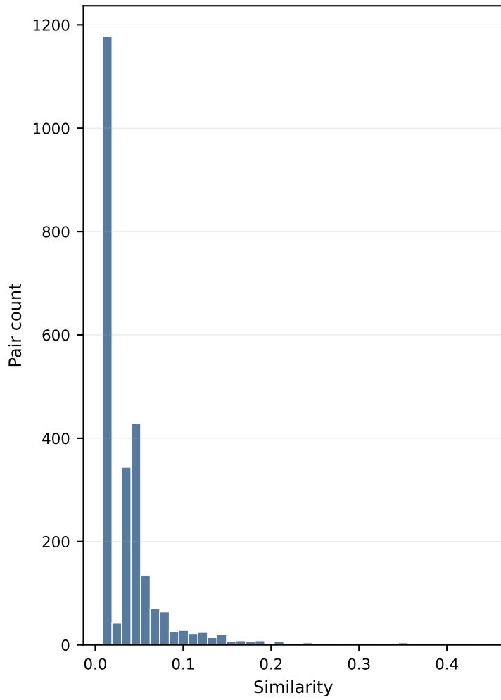
Off-diagonal similarities
