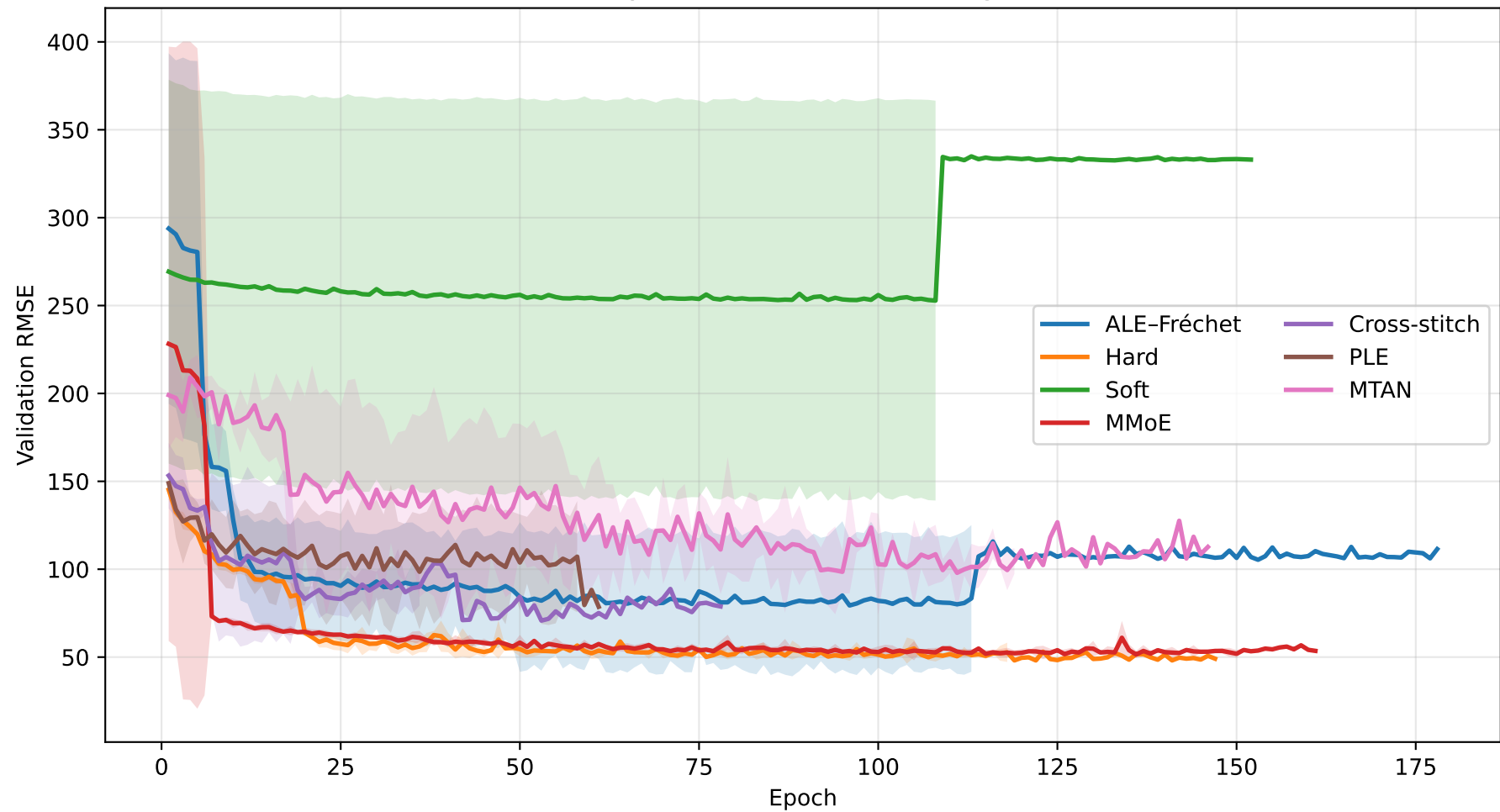
electricity: Validation RMSE learning curves
