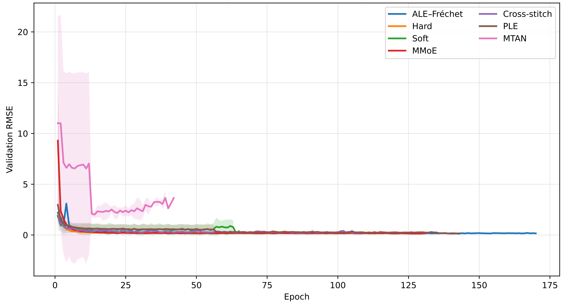
exchange: Validation RMSE learning curves
