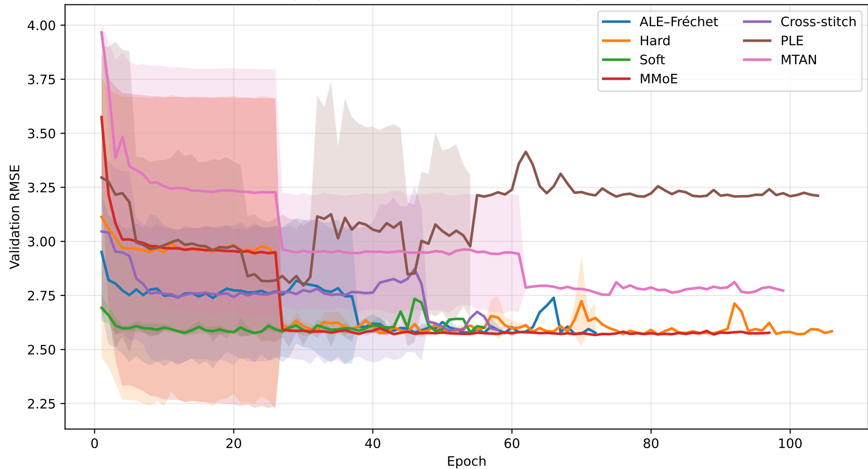
polynomial: Validation RMSE learning curves
