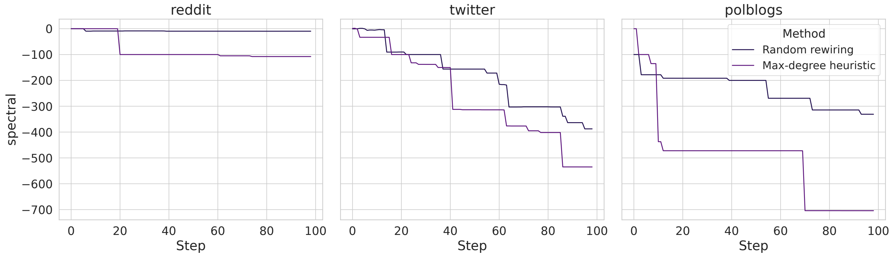
Fiedler \lambda_2 percent change vs step (baselines)
