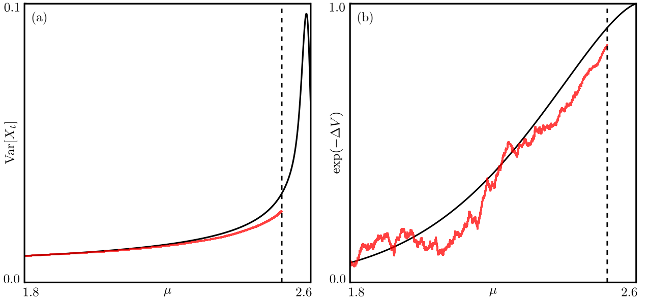
Figure 7: Comparison between the increase in variance and modified escape EWS applied to a slowly ramped model of ecosystem collapse (23), introduced in [43]. We fix parameters r = 1 , k = 10 and h = 1 while we let \mu to vary between 1.8 and 2.6 with rate \varepsilon = 5 \cdot 10^{-5} ; the bifurcation diagram of the stationary system is reported in Figure 2(a). A simulation of 100 sample paths allows us to compute ensemble averaged variance and modified escape EWS (both in red) on a sliding window of 10% the length of the solutions. In each panel the accuracy of empirical signals is compared to the approximations of the stationary system (both in black). The earliest tipping in the solutions is shown by the dashed line. Notice how both variance and modified escape EWS show upward trends in the approach to the tipping point. The increase in variance however requires the knowledge of a baseline value which is different from that of other systems (e.g. see Figure 6(c)) while the increase in escape likelihood shows a more reliable, direct interpretation as an EWS.
