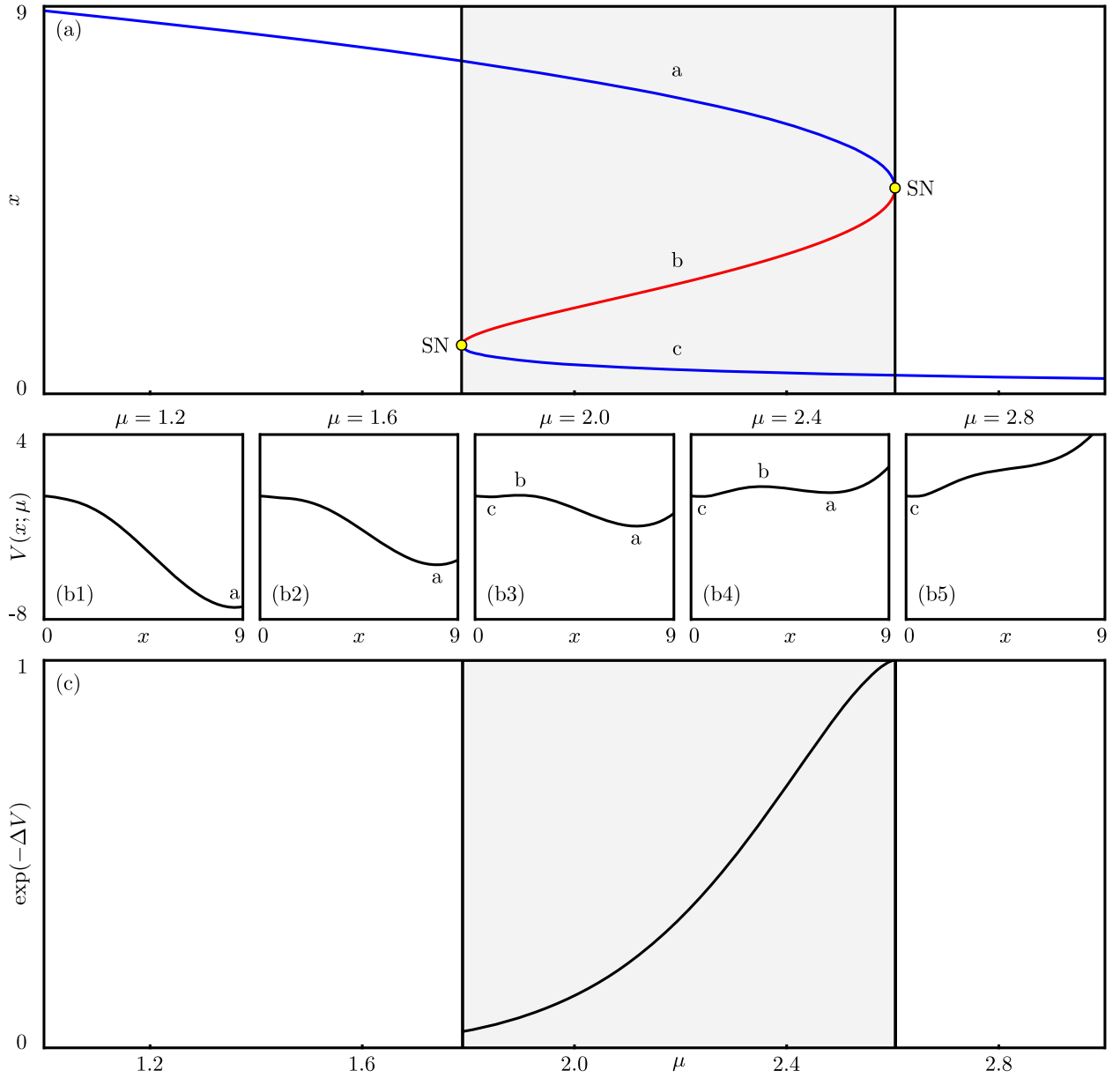
Figure 2: (Panel (a)) Bifurcation diagram of a model of ecosystem collapse with the state x (vegetation biomass) degrading as the forcing parameter \mu (harvesting rate) is increased [43]; branches of stable equilibria ( x = a and x = c ) are in blue while the unstable branch ( x = b ) is in red; the region of bistability, bounded by two SN bifurcations (yellow circles), is shaded in gray. (Panels (b1-b5)) Different configurations of the potential V(x; \mu) = -\frac{x^2}{2} + \frac{x^3}{30} + \mu(x - \arctan(x)) at different parameter values (ticks of the horizontal axes of panels (a) and (c)). (Panel (c)) Modified escape EWS (4) computed out of the potential V(x; \mu) between the stable state x = a and the saddle x = b within the bistability region. The bifurcation diagram has been computed using the BifurcationKit.jl package [63].
