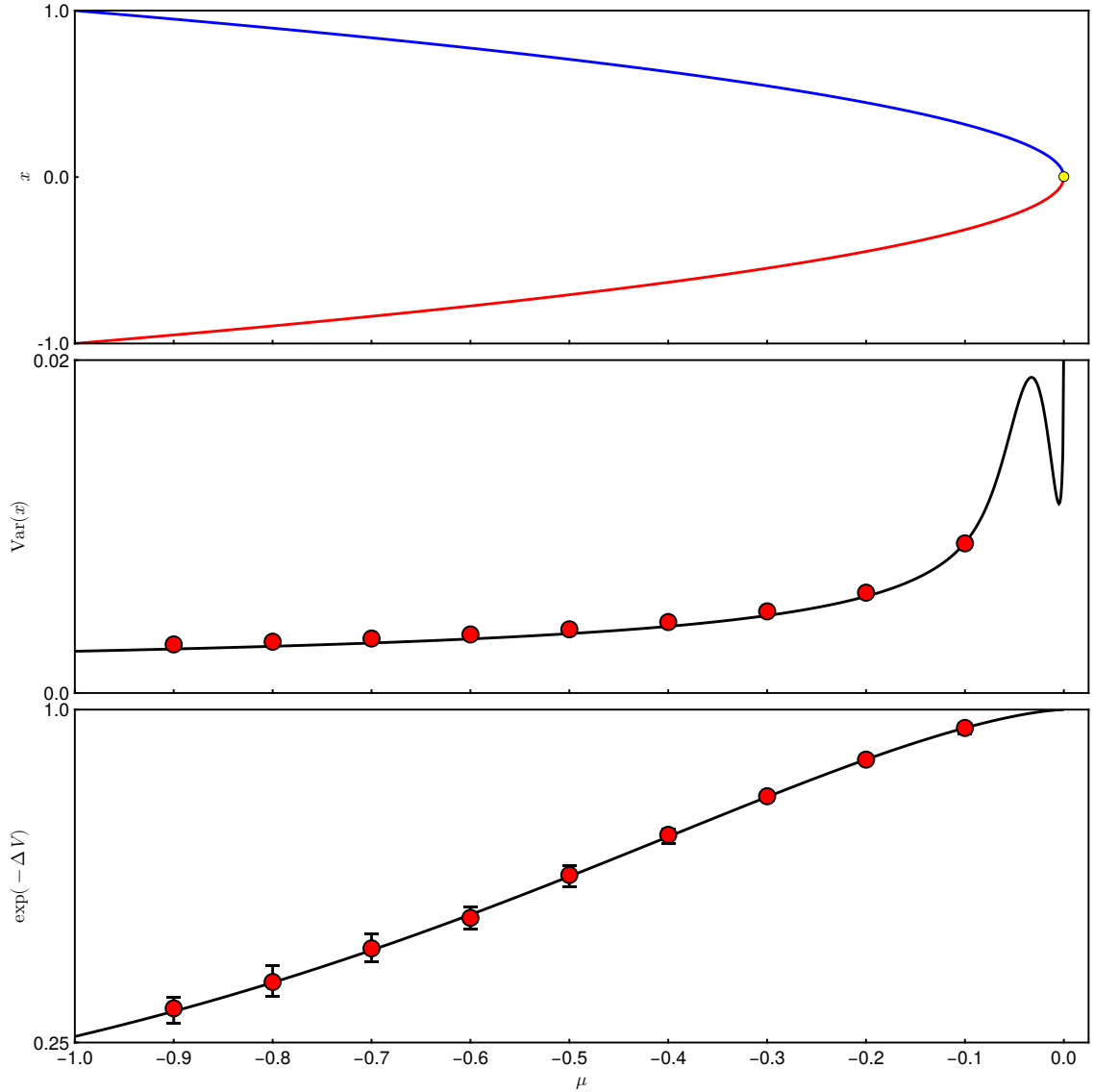
Figure 5: Comparison between the increase in variance and modified escape EWS for stationary solutions of a SN normal form at different values of the bifurcation parameter \mu \in [-1, 0] . In the top panel the bifurcation diagram is shown with the blue curve representing the branch of the stable equilibrium a = \sqrt{-\mu} while the red curve represents the unstable equilibrium branch b = -\sqrt{-\mu} ; the SN bifurcation is depicted by the yellow circle at \mu = 0 . In the middle and bottom panels we compare the analytical (black curves) and empirical (red circles) variance and modified escape rate respectively. The analytical values have been computed using 20 for the variance and 6 for the escape EWS; the empirical values have been computed by taking the median of an ensemble of 100 sample paths at each parameter value. The error bars represent the interquartile range of the compute quantity. Notice how, alongside interpretability, the modified escape EWS is also “earlier” in the upward trend compared to the increase in variance which furthermore shows non-monotonicity at the very onset of the B-tipping event causing potential false negatives.
