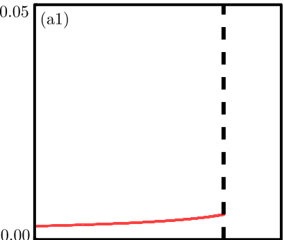
SN normal form
