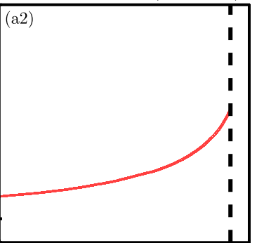
Ecosystem collapse (May, 1977)
