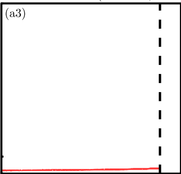
Ocean circulation (Stommel, 1966)
