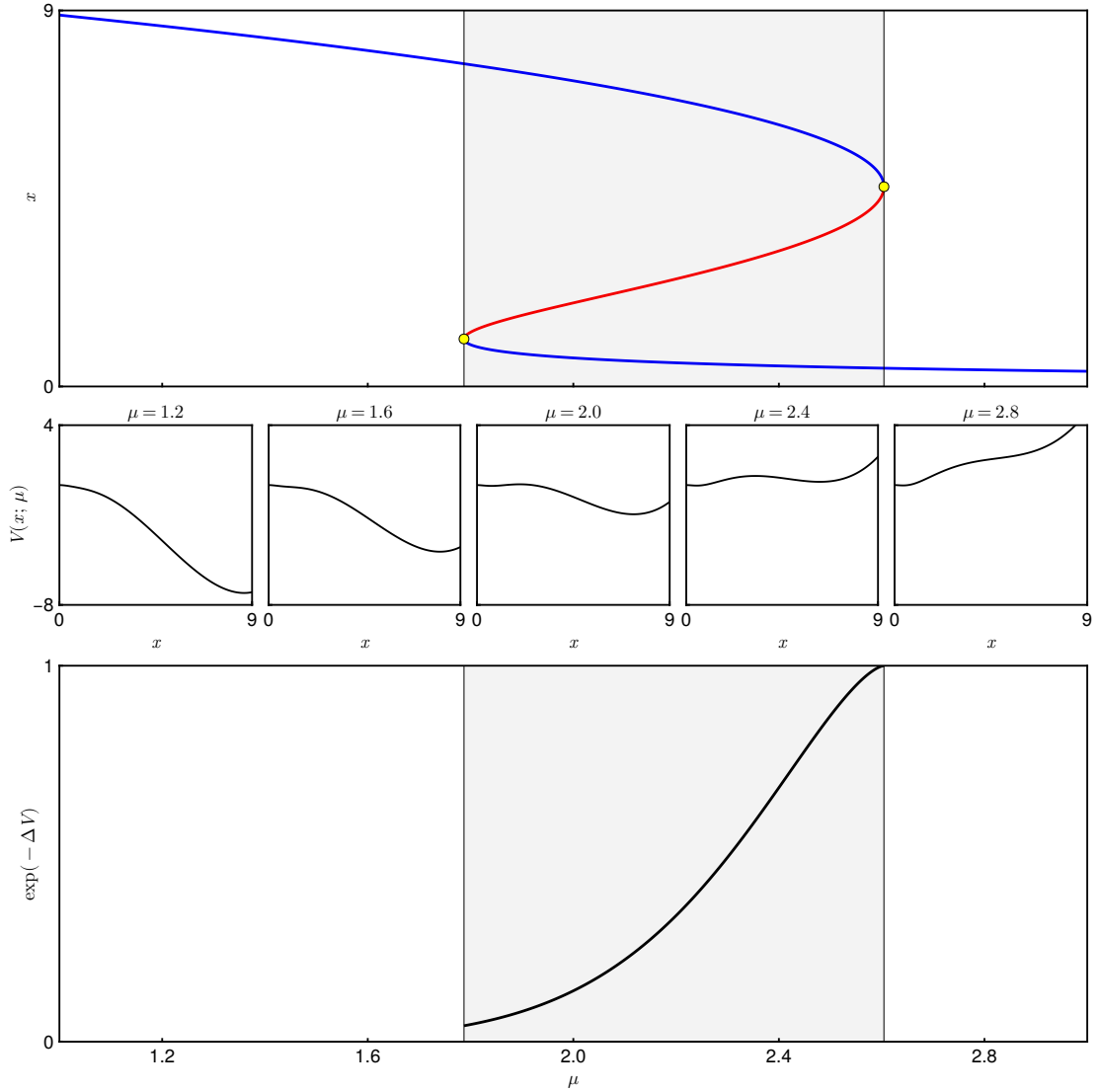
Figure 2: (Top): bifurcation diagram of a model of ecosystem collapse with the state x (biomass) degrading as the forcing parameter \mu (harvesting rate) is increased [8]; branches of stable equilibria ( x = a and x = c ) are in blue while the unstable branch ( x = b ) is in red; the region of bistability, bounded by two SN bifurcations (yellow dots), is shaded in gray. (Middle) Different configurations of the potential V(x; \mu) of the system at different parameter values corresponding to the ticks of the horizontal axes of the top and bottom plots. (Bottom) Modified escape EWS computed out of the potential V(x; \mu) between the stable state x = a and the saddle x = b within the bistability region.
