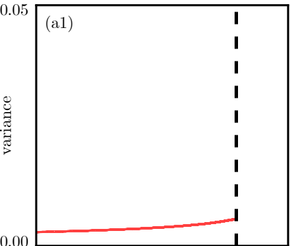
Saddle-node normal form
