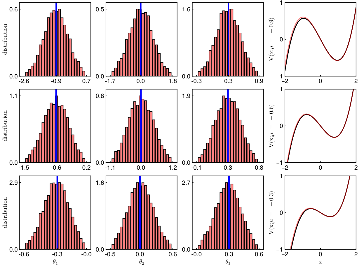
Figure 4: Distribution of the solutions \theta^* = (\theta_1^*, \theta_2^*, \theta_3^*) of the LLS regression problem for a SN normal form with drift f(x; \mu) = -\mu - x^2 . The problem is solved for different configurations of the potential at different values of the bifurcation parameter; at \mu = -0.9 the system is far from the bifurcation (top row); at \mu = -0.6 the system is closer to the bifurcation (middle row); at \mu = -0.3 the system is very close to the bifurcation. For each configuration we compute an ensemble of solutions of 19, represented by the normal shaped histograms, using 5,000 sample paths of the normal form at their respective parameter value. The value of the polynomial coefficients of the true potential V(x; \mu) = \mu x + \frac{x^3}{3} are displayed, in each box, by a blue line. The (ensemble) mean values of the LLS solutions \hat{\theta}^* = (\hat{\theta}_1^*, \hat{\theta}_2^*, \hat{\theta}_3^*) are then used to plot an ensemble mean reconstruction of the potential \hat{V}_*(x) := V(x; \hat{\theta}^*) = \sum_{k=1}^3 \hat{\theta}_k^* x^k (depicted in red in the leftmost boxes) and compared with the ground truth (in black). Notice the consistency in accuracy for the mean reconstruction.
