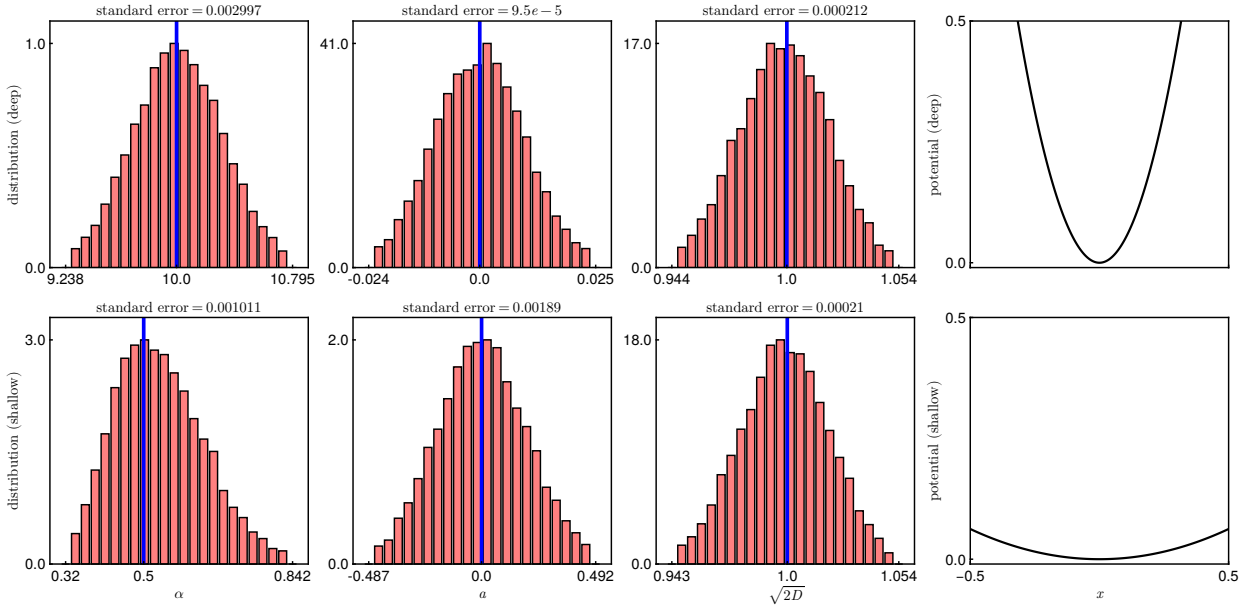
Figure 3: Empirical distribution of the MLE of the parameters \theta = (\alpha, a, D) of an ensemble of 10,000 sample paths solving 14 for two different configurations of the potential V(x) = \alpha(a - x)^2 : a deep, strongly confined well with \alpha = 10 (top row); a shallow well with \alpha = 0.5 (bottom row). In each of the plots the true value of the parameter used to generate the data is depicted (blue line) while at the top we report the standard error of the distribution. Notice how, as the SN bifurcation of the linearised vector field is approached \alpha = f'(x = a) \rightarrow 0 , the distribution of the estimators of the linear coefficient becomes more skewed despite the symmetry in the confining potential. These solutions have been computed using the pymle package [21].
