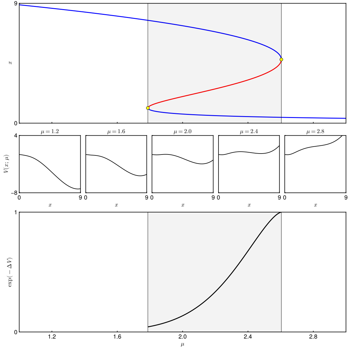
Figure 2: (Top): bifurcation diagram of a model of ecosystem collapse with the state x (biomass) degrading as the forcing parameter \mu (harvesting rate) is increased [27]; branches of stable equilibria ( x = a and x = c ) are in blue while the unstable branch ( x = b ) is in red; the region of bistability, bounded by two SN bifurcations (yellow dots), is shaded in gray. (Middle) Different configurations of the potential V(x; \mu) of the system at different parameter values corresponding to the ticks of the horizontal axes of the top and bottom plots. (Bottom) Modified escape EWS computed out of the potential V(x; \mu) between the stable state x = a and the saddle x = b within the bistability region. The bifurcation diagram has been computed using the BifurcationKit.jl package [39].
