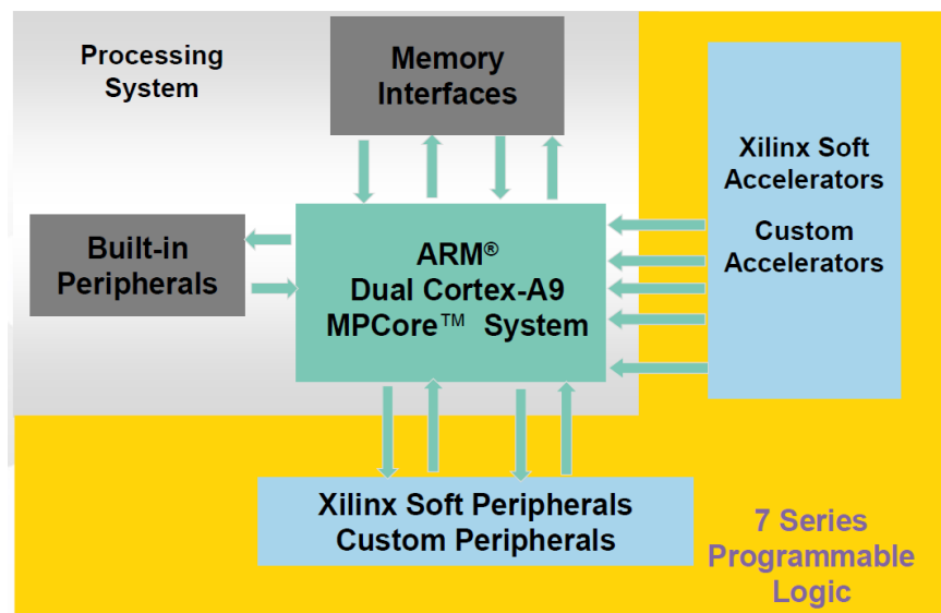
Figure 1. Simplified model of the Zynq architecture.
