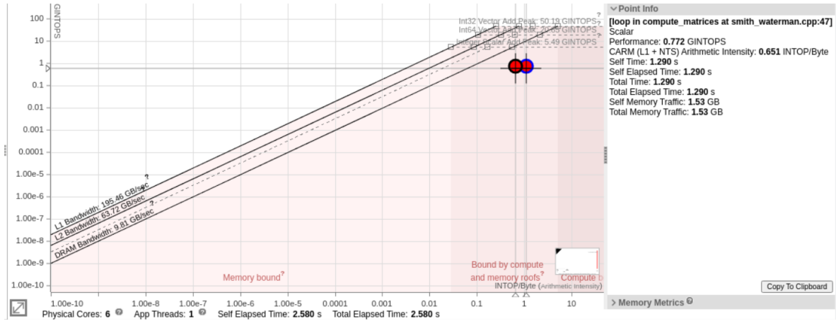
Figure 6. Roofline chart of the LSAL compute kernel executed on an x86 6-core CPU as shown by Intel Advisor tool. The two red dots correspond to the execution of the compute_matrices function for the L1-based arithmetic intensity (dot to the left) and the DRAM-based arithmetic intensity (dot to the right). The L1-based AI is equal to \frac{\#INT\ Ops}{\#bytes\ read\ from\ L1\ DCache} , whereas the DRAM-based AI is equal to \frac{\#INT\ Ops}{\#bytes\ read\ from\ DRAM} . Since the \#bytes\ read\ from\ DRAM in a CPU is typically much lower than the \#bytes\ read\ from\ L1\ DCache , the DRAM-based AI is usually larger. As we can see, multiple values can characterize AI in a CPU with a memory hierarchy. Note also the multiple horizontal rooflines which correspond to the maximum performance for Integer scalar 32/64 bits and Int32 vector.
