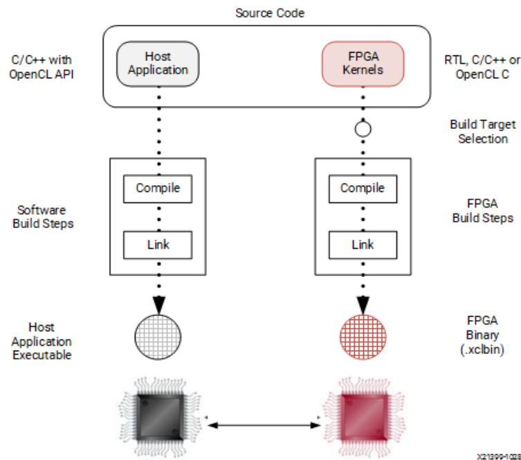
Figure 7. Software/Hardware Build Process
