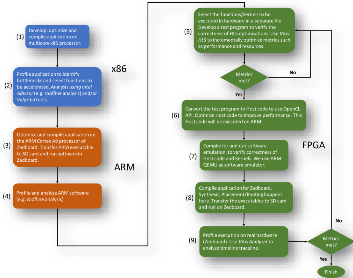
Figure 2. Development flow of lab3. The numbers in parentheses correspond to the material in the subsections of section 3.
