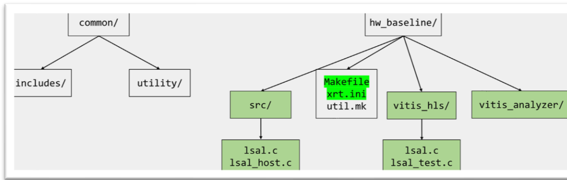
Figure 3. Directory structure used in this lab for application development. The files and/or directories you need to modify are colored in green. For each new kernel implementation, you need to build a new directory structure like hw_baseline . The development starts with the Vitis HLS, and then the lsal.c file has to be copied over to the src/ directory.
