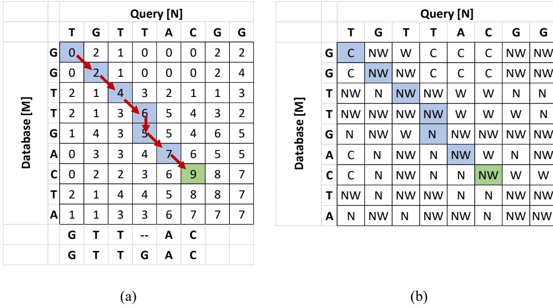
Figure 1. (a) LSAL Similarity matrix for a Database of length M=9 , and a Query of length N=8 . The cell with the largest similarity value, when the algorithm terminates, is shown in Green. We start searching for the longest local sequence alignment (shown at the bottom of the similarity matrix) starting from this cell and backtracing till we reach a cell with a value of 0 in the similarity matrix. Note that the alignment is partial since the last G of the database does not match the symbol of the query. (b) The corresponding direction matrix. Note that the priority among the four possible directions in case of a draw is C, NW, N, W. Note that, in most cases, the database length M is much larger than the query length N , i.e. M \gg N . T = Thymine, G = Guanine, A = Adenine, and C = Cytosine are the four main nucleobases found in the nucleic acids DNA and RNA.
